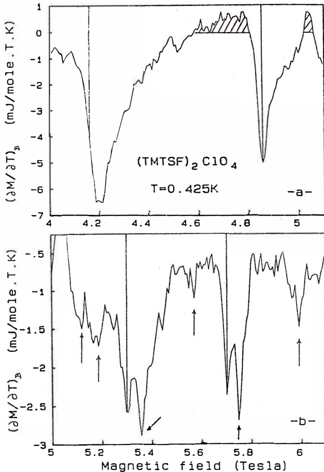
Figure 2: Magnetocaloric effect plotted versus the magnetic field. Vertical lines feature "integer" transitions between FISDWs, dashed areas represent positive entropies associated with partial reentrances, and arrows display the fractional doublets.
