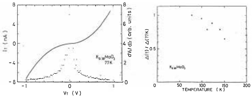
Fig. 1 Tunneling current I_T vs. tunneling voltage V_T (solid line) and dV_T/dI_T vs. V_T (solid circle).
