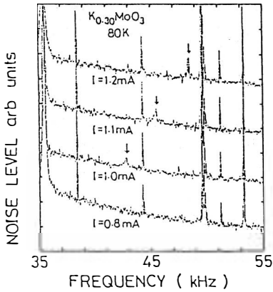
Fig. 3 Spectra of tunneling current under transport current. For current exceeding the threshold value ( I_c=0.95 mA), a new peak (indicated by arrows) appears in the current spectra.
