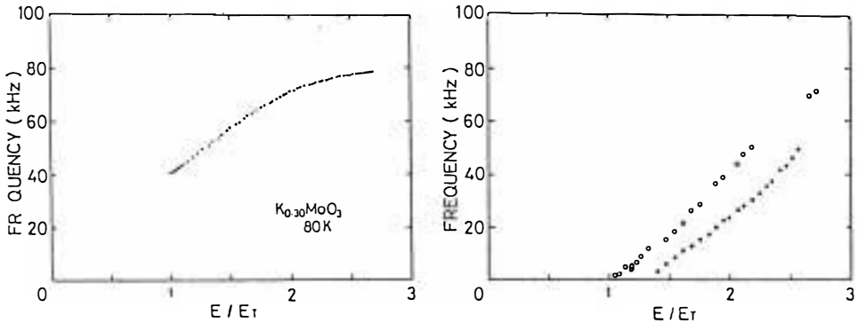
Fig. 4 Peak frequency in the tunneling current spectra vs. transport voltage.
