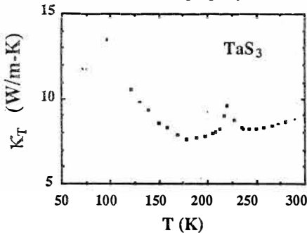
FIG.2 – Thermal conductivity of \text{TaS}_3 measured by a self-heating method.
