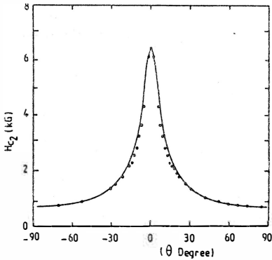
Fig. 3 - Angular dependence of H_{c2} of (PbS)_{1.14}NbS_2 at T = 2.14 K. The curve is the fit with Equat. 1 with \epsilon = 8.97 .
