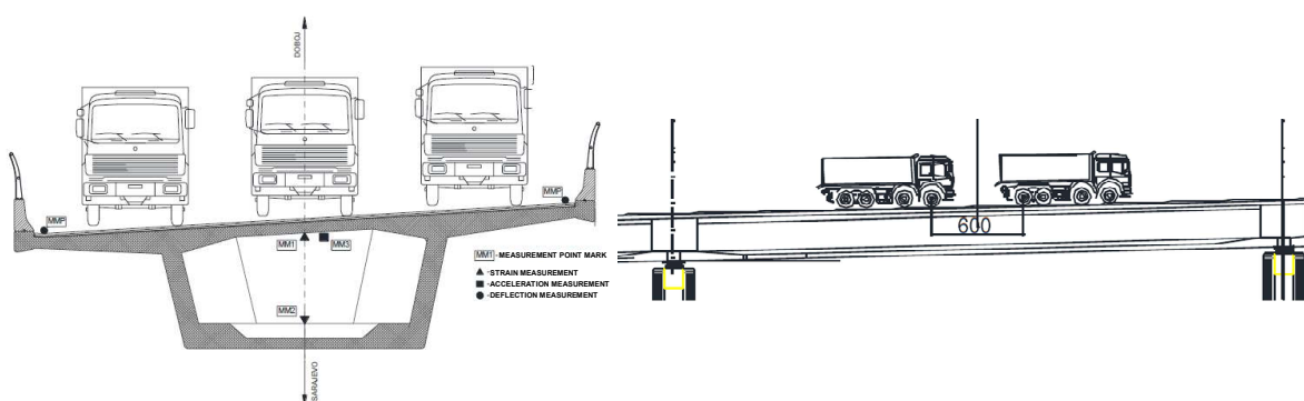
Figure 3. – Position of the trucks in the cross section Figure 4. – Longitudinal position
