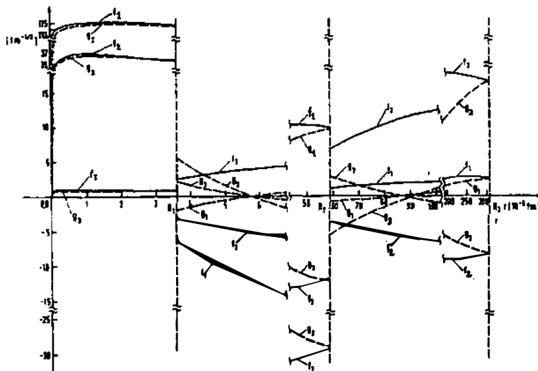
Fig. 2. The radial dependence of the upper components f_i (full lines) and of the lower components g_i (dotted lines) of the three wave functions corresponding to the energies E_i . The three vertical dashed lines indicate the positions of the two delta functions and the infinite wall, respectively.
