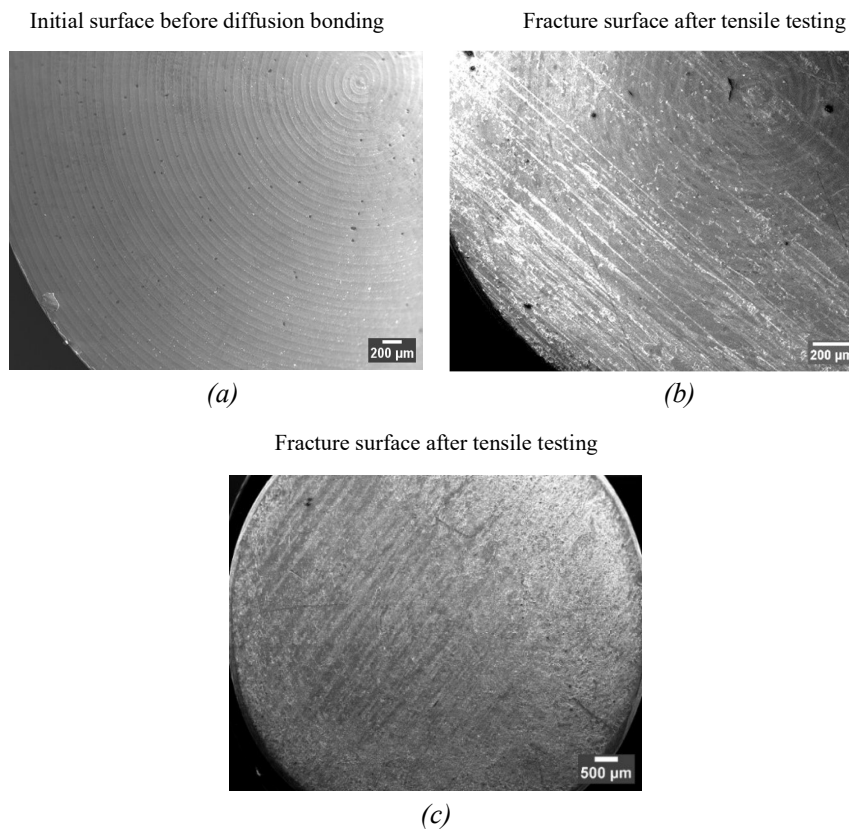
Figure 6. SEM micrographs of: (a) initial surface of AA7075-T6, (b) fracture surface of AA7075-T6 diffusion bonded at 475°C-40MPa-5s after tensile testing, and (c) fracture surfaces of AA7075-T6 diffusion bonded at 500°C-15MPa for holding time of 30 s.
