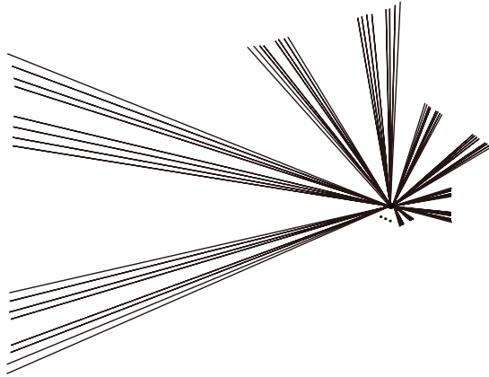
FIGURE 3.1. The star of Cantor fans
