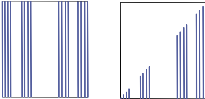
FIGURE 3.2. The spaces P and R
