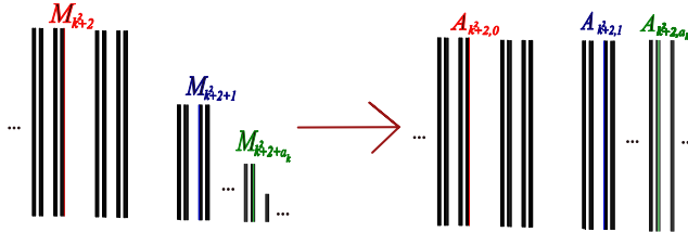
FIGURE 4.5. The arcs A_{k,i} in C \times [0, 1]
