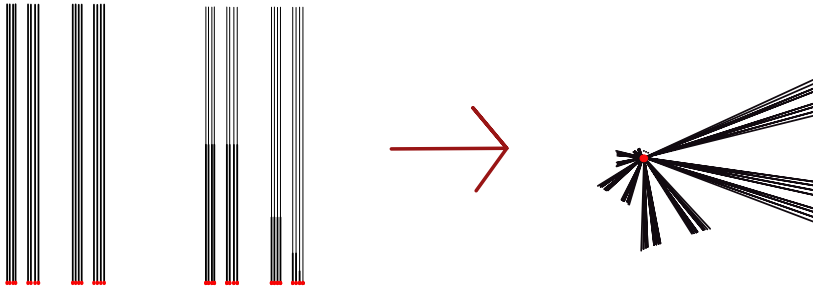
FIGURE 4.3. The relation \approx from Definition 4.40
