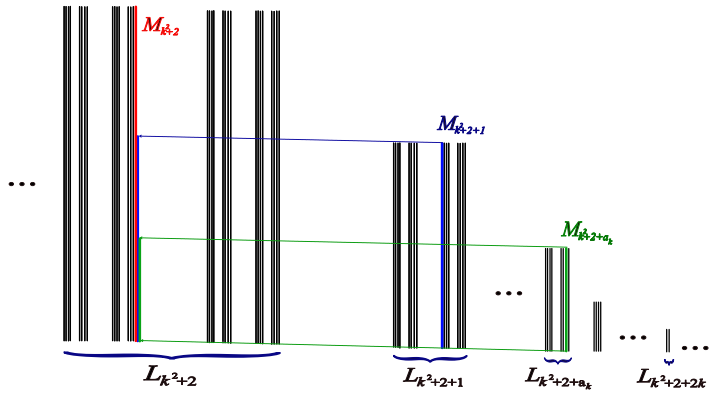
FIGURE 4.4. The relation \approx_{\mathbf{a}} from Definition 4.40
