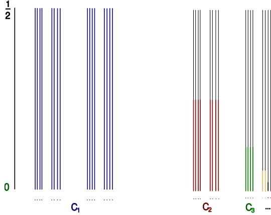
FIGURE 4.2. The space \left(\bigcup_{k=1}^{\infty} \left(C_k \times \left[0, \frac{1}{2^{2k-1}}\right]\right)\right) \cup \{(1, 0)\}
