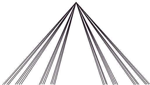
FIGURE 2.1. A Cantor fan
