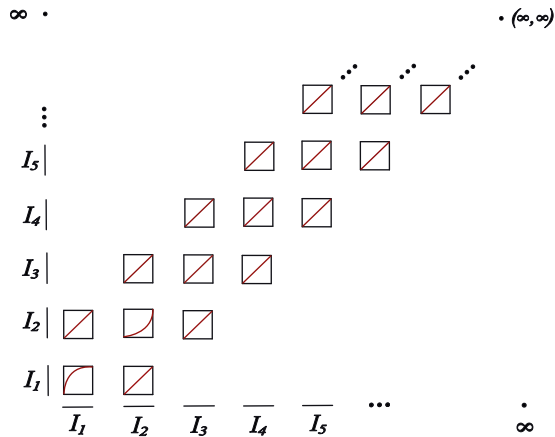
FIGURE 4.1. The relation H on \mathbb{X}
