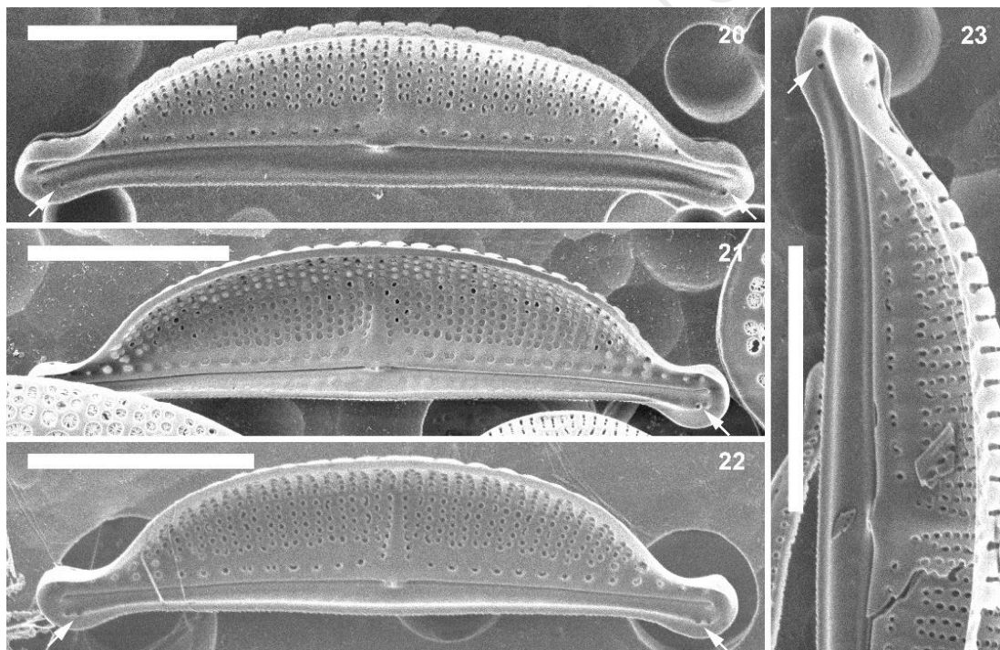
Pl. 2. SEM internal views of Halamphora yundangensis (Figs. 20–23) from populations on a loggerhead sea turtle’s carapace (Figs. 20, 23, Adriatic Sea, sample TB225, stub BR-4916) and on macroalgae (Figs. 21, 22, Adriatic Sea, samples ENV10, s.n., and ENV14, stub BR-4873, respectively). White arrows indicate the poroids at the apices. Scale bars = 5 \mu\text{m} . SEM – Scanning electron microscopy.
