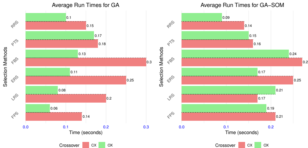
Figure 2: Ranking of Selection methods by average run times.
