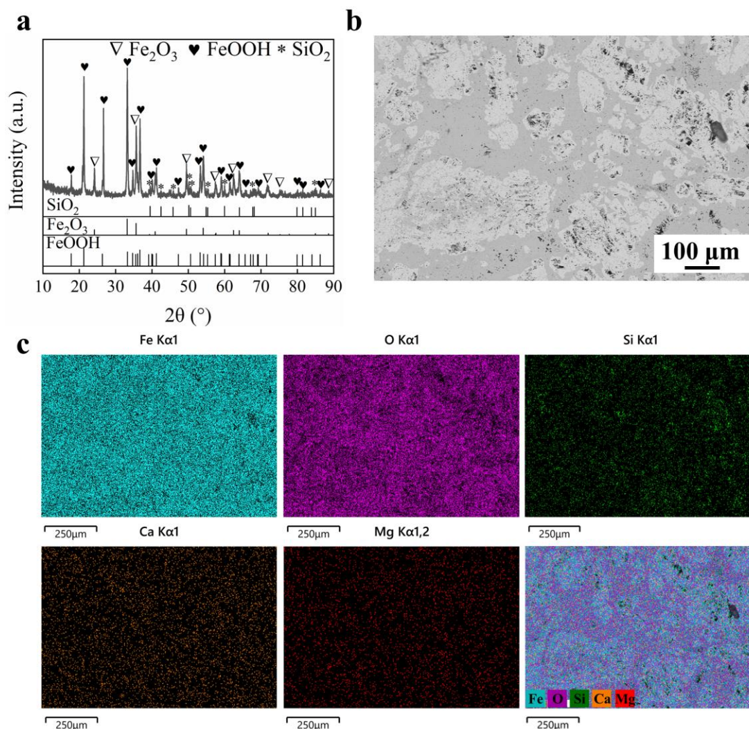
Figure 1. (a) XRD pattern, (b) SEM analysis and (c) EDS mapping results of L1.
