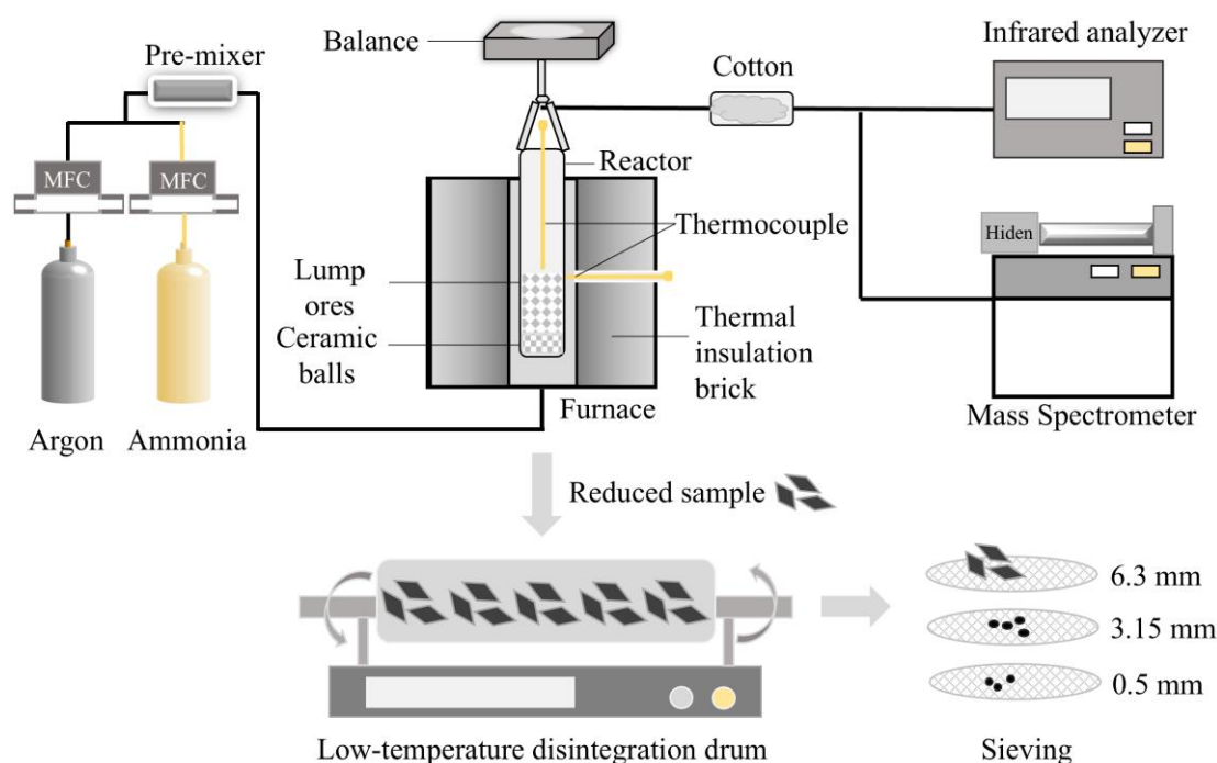
Figure 2. Schematic diagram of experimental setup and process.
