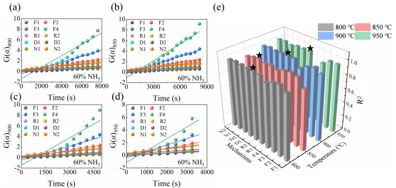
Figure 10. Results of linear fitting between G(\alpha) and t during 60 % NH 3 reducing L1 by the model-fitting method at different reduction temperatures: (a) 800 °C, (b) 850 °C, (c) 900 °C, and (d) 950 °C. (e) The R^2 value of the fitted lines in Figure 10(a), Figure 10(b), and Figure 10(c), and Figure 10(d). (★ denotes the mechanism with the highest R^2 )
