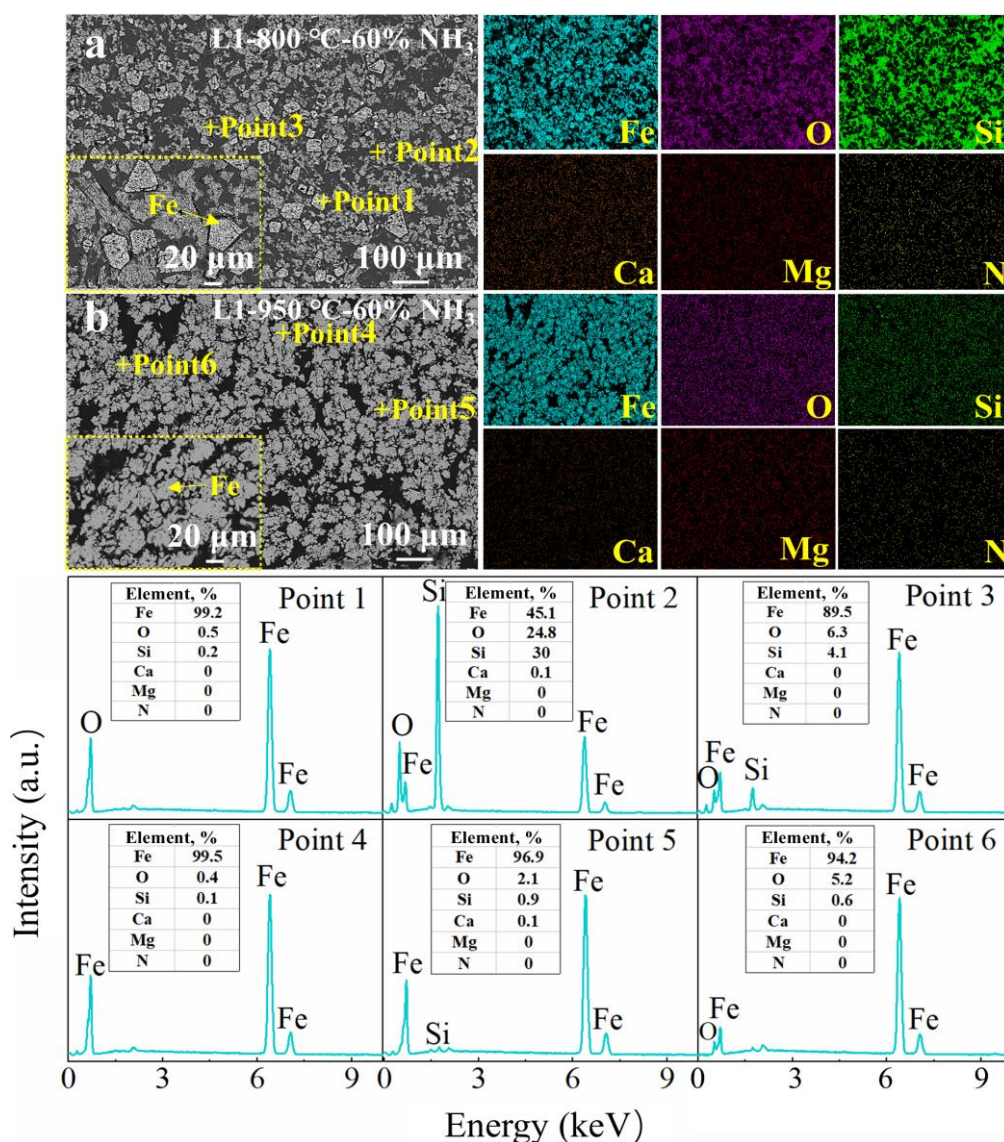
Figure 4. SEM-EDS analysis of the reduced samples: (a) L1-800 °C-60 % NH 3 , and (b) L1-950 °C-60 % NH 3 .
