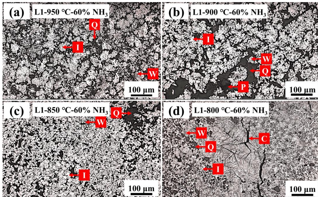
Figure 5. OM analysis of the reduced samples under different temperatures: (a) L1-950 °C-60 % NH 3 , (b) L1-900 °C-60 % NH 3 , (c) L1-850 °C-60 % NH 3 , and (d) L1-800 °C-60 % NH 3 . (P: pore. Q: quartz. C: crack. I: Fe. W: wüstite.)
