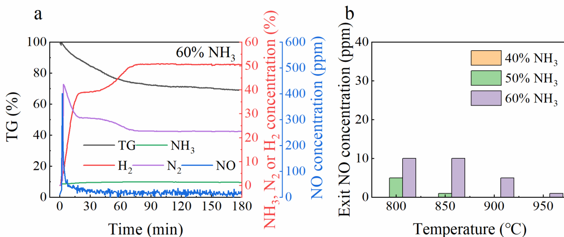
Figure 6. (a) TG curves and outlet gas concentrations change during the reduction of L1 by 60 % NH 3 at 900 °C. (b) Variation in NO concentration at the outlet during the reduction of L1 at 180 minutes with different concentrations of NH 3 within the temperature range of 800 °C–950 °C.
