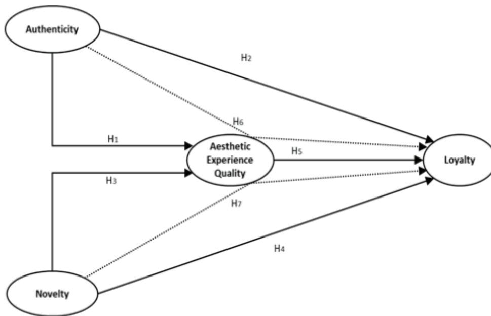
Figure 1: Research Model
