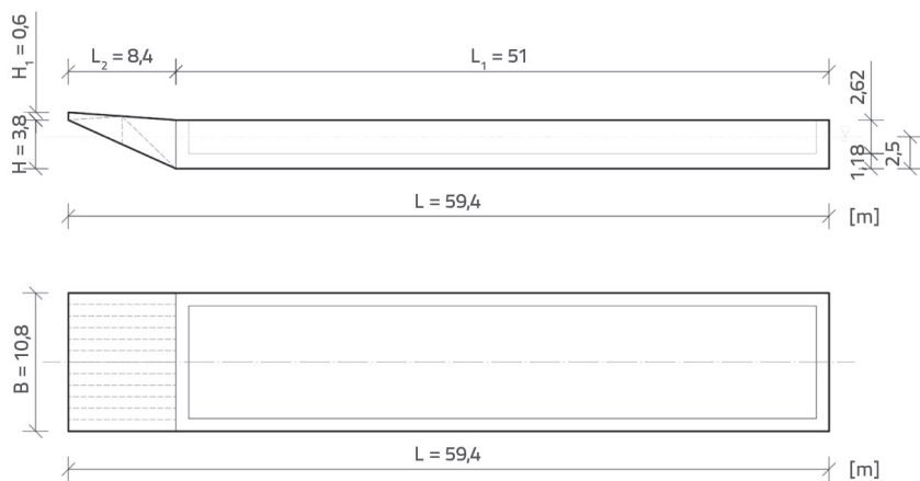
Figure 8. Barge geometry
