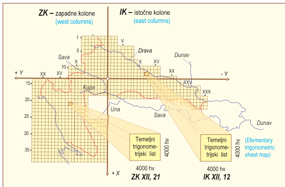
Fig. 28. Division into base trigonometric sheets in the Kloštar Ivanić Coordinate System (according to Macarol, 1977)
