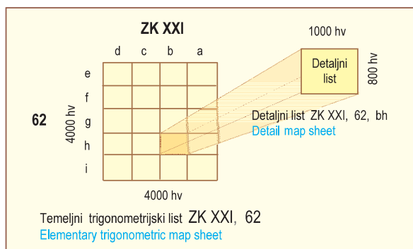
Fig. 22. Division of base trigonometric sheets in the Budapest Coordinate System, 4000 fathoms × 4000 fathoms into detailed sheets (sections), 1000 fathoms × 800 fathoms
