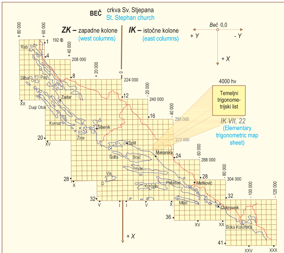
Fig. 18. Division into basic trigonometric sheets in the Viennese Coordinate System for the first cadastral survey in Dalmatia and Boka Kotorska. Columns are marked with Roman numbers, and rows with Arabic numbers. Coordinates of a certain number of trigonometric sheet edges are expressed in fathoms (according to Borčić and Frančula, 1969)
