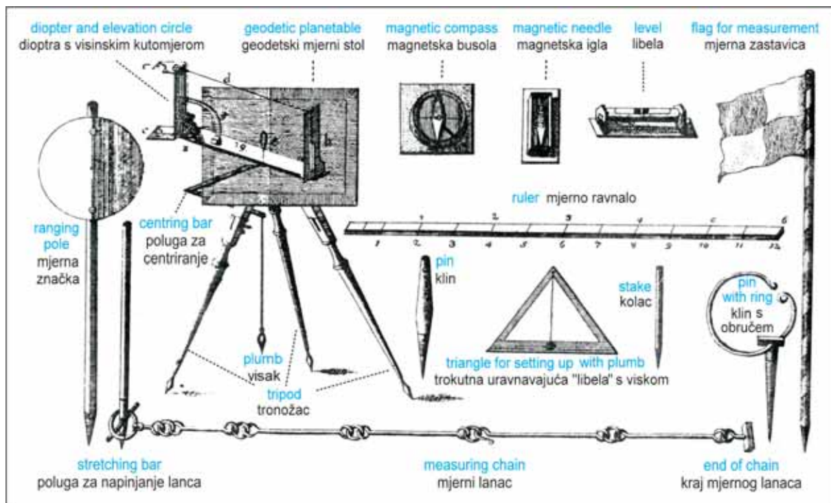
Fig. 10. Surveyor's tools of the late 18th century, according to Lang's manual from 1804 (Korošec 1978, page 136). A pair of compasses with two spikes, i.e. tools for drawing and mapping points should be added.
