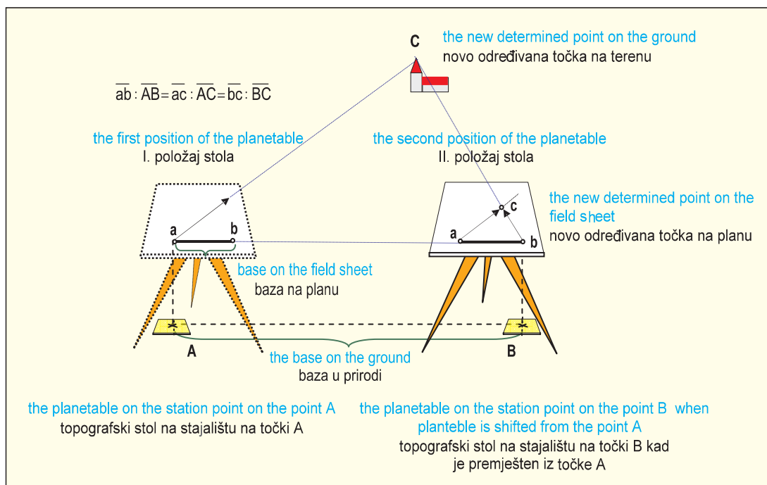
Fig. 11. A clear representation of field mapping by a forward intersection with a plane table (Praetorius surveying table) from points A and B. The point C was determined. In point A, the table is oriented toward point B and a straight line is drawn toward point C, and in point B, the table is oriented toward point A and a straight line is drawn toward point C. The new point is at the intersection of the two straight lines. On the horizontal plane table, one can see in point B that horizontal length in nature between points A, B and C are proportional to length on the plan of the planetable between points a, b and c. The scale of the produced plan is the scale of base relations, plan base and base in nature.
