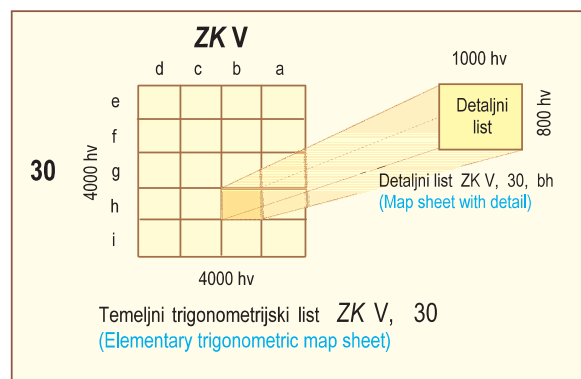
Fig. 15. Division of basic trigonometric sheet with dimensions 4000^{\circ} \times 4000^{\circ} into detailed sheets (sections) with dimensions 1000^{\circ} \times 800^{\circ}
