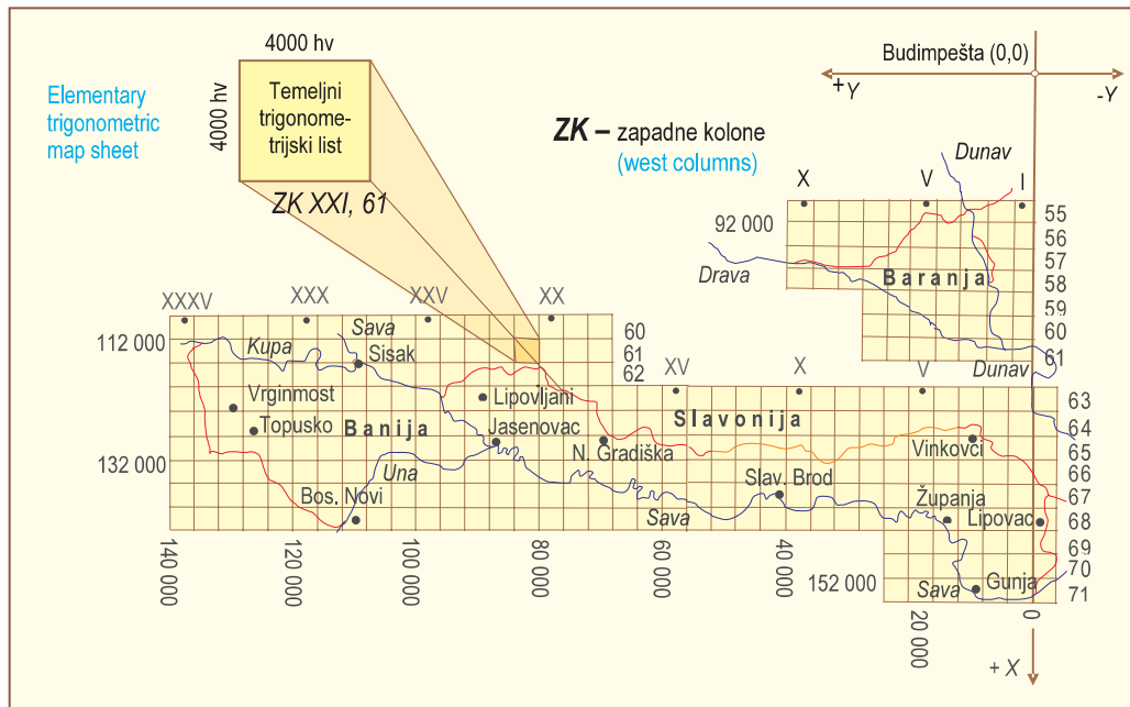
Fig. 21. Division into base trigonometric sheets of Baranja and part of the area of the Military Border Regiments (south Slavonia and Baranja) without six western Regiments, which were included into coordinate system with the origin in the Gellérthegy trigonometric point (Budapest) (according to Borčić and Frančula, 1969)
