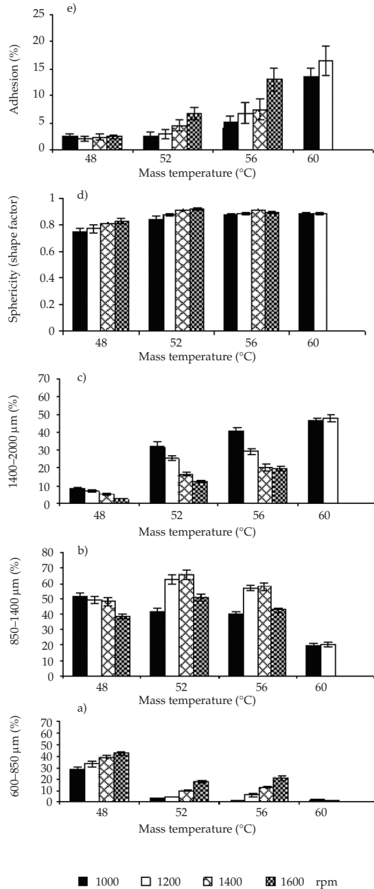
Fig. 2. Effect of mass temperature and friction plate speed on pellet characteristics at bowl temperature of 45 °C and 40 % ( m/m ) wax concentration (mean ± SD, n = 3).
