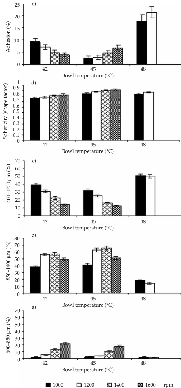
Fig. 1. Effect of bowl temperature and friction plate speed on pellet characteristics at mass temperature of 52 °C and 40 % ( m/m ) wax concentration (mean ± SD, n = 3).
