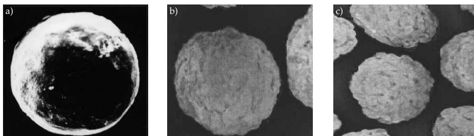
Fig. 4. SEM photographs of: a) 2000 µm, b) 1400 µm and c) 850 µm pellets at 25x magnification.
