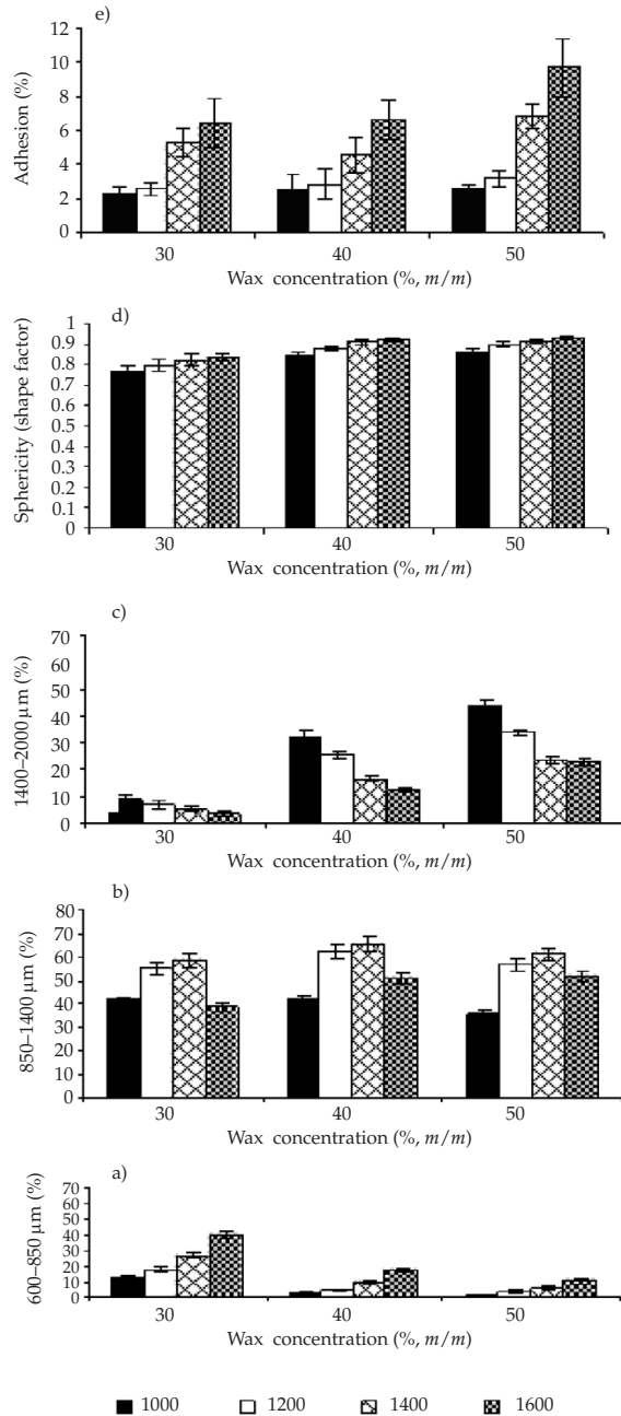
Fig. 3. Effect of wax concentration and friction plate speed on pellet characteristics at bowl temperature of 45 °C and mass temperature of 52 °C (mean ± SD, n = 3 ).
