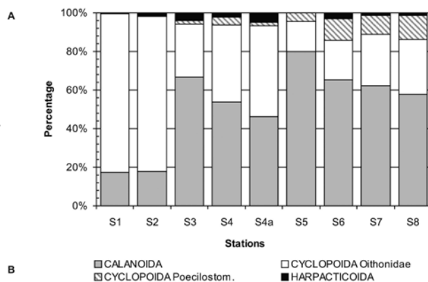
Fig. 8. Percentage contribution of the copepod orders to total copepod abundance in the 125- \mu\text{m} taxocenosis
