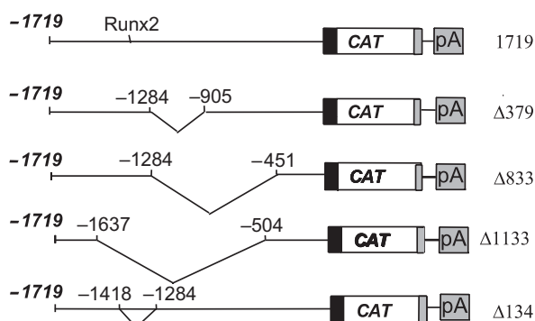
Fig. 1. Internal deletions of ColCAT1719. Constructs were named by the number of deleted base pairs: \Delta 379, \Delta 833, \Delta 1133 and \Delta 134. The Runx2 binding at –1376 bp is shown.
