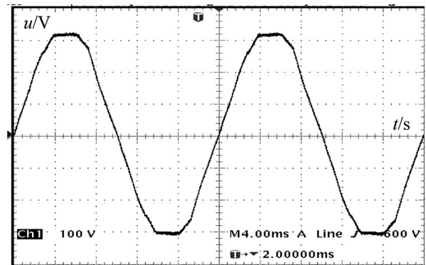
Fig. 11 Supply voltage
