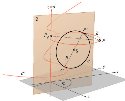
Figure 2: One system of the curves on \mathcal{P}_n^{n+2} can be constructed as circles in the planes through d with the end points of the diameters on c^n and k .
