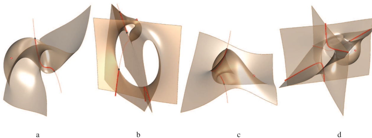
Figure 22: Figure a – \mathcal{PK}_3^5 type I for P(4, 4, 0) ; figure b – \mathcal{PK}_3^5 type II for P(2, -1, 3) ; figure c – \mathcal{PK}_3^5 type III for P(1, 2, 0) ; figure d – \mathcal{PK}_3^5 type IV for P(5, -1, 3) .
