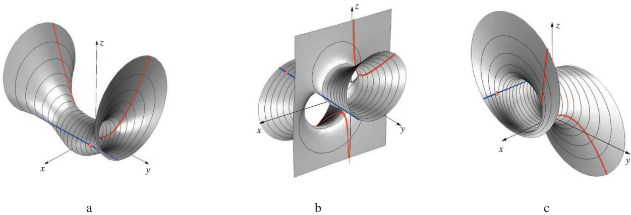
Figure 16: a – \mathcal{D}_1^3 defined by d^\infty in the plane y = 0 , c^2 given by equations x = 0 and z = \frac{y^2}{2} and P(2, 1.5, 1) . b – \mathcal{D}_1^3 defined by d^\infty in the plane y = 0 , c^2 given by equations x = 0 and y^2 - yz + 1 = 0 and P(3, -4, 1) . c – \mathcal{D}_2^4 defined by d^\infty in the plane x = 0 , c^3 given by equations y = \frac{x^2}{5} and z = \frac{x^3}{10} and P(3, -4, 2) .
