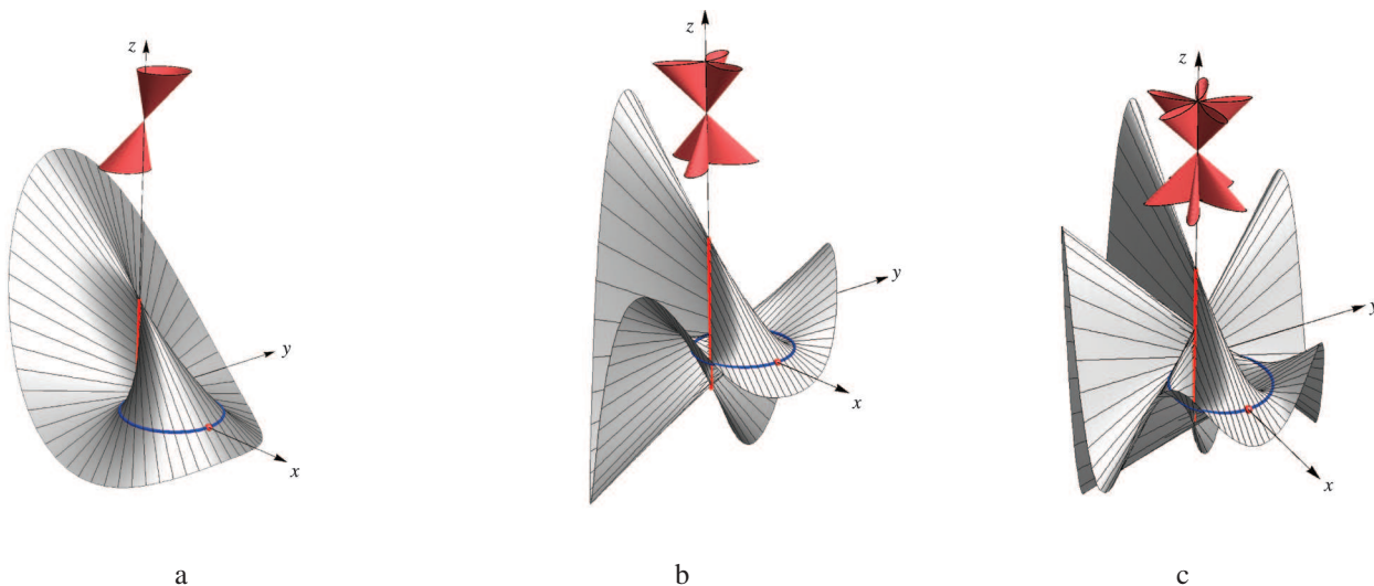
Figure 17: The pedal ruled surfaces for the pole P(2, 0, 0) , axis z and 1, 3 and 5-petalled roses in the plane at infinity are shown in figures a, b and c, respectively. These directing roses are the curves at infinity of the highlighted red cones.
