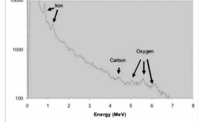
Figure 13 Gamma spectrum from 5 kg of TNT behind the iron plate 16 mm thick ( 12 \times 10^7 tagged neutrons, measurement time 3490 s); logarithmic scale – bottom; linear scale – top
