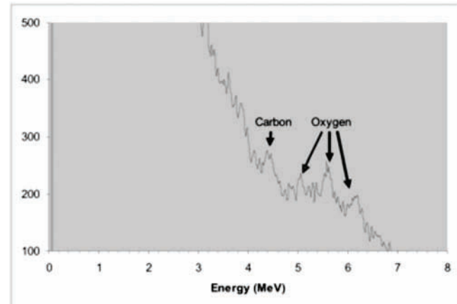
Figure 13 Gamma spectrum from 5 kg of TNT behind the iron plate 16 mm thick ( 12 \times 10^7 tagged neutrons, measurement time 3490 s); logarithmic scale – bottom; linear scale – top
