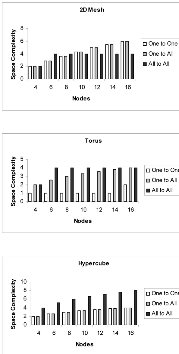
Figure 8. Comparison of space complexities.
