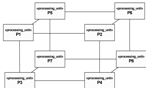
Figure 3c. UML class diagram of hypercube topology.
