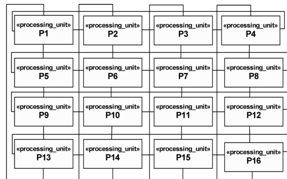
Figure 3b. UML class diagram of torus topology.
