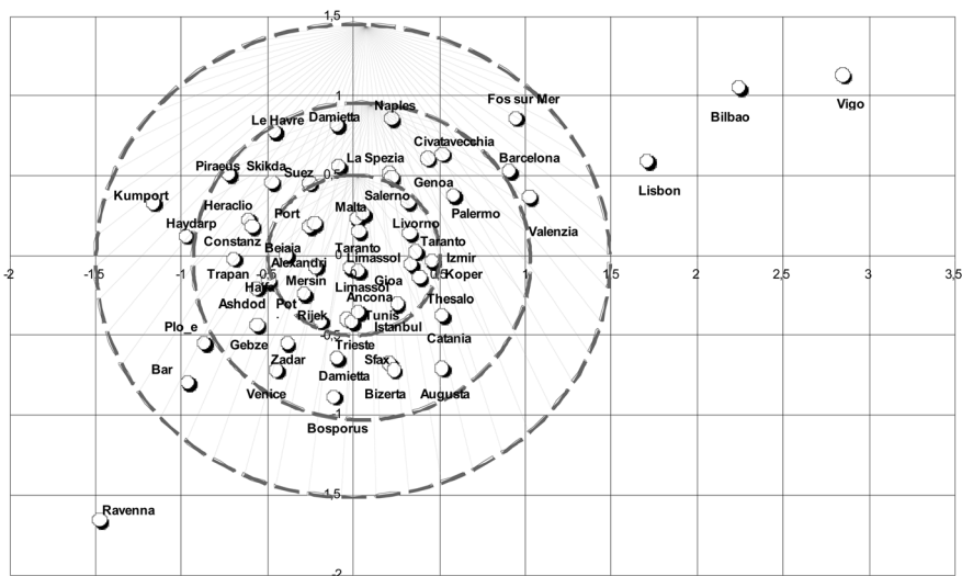
Fig. 5 Multidimensional scalling
