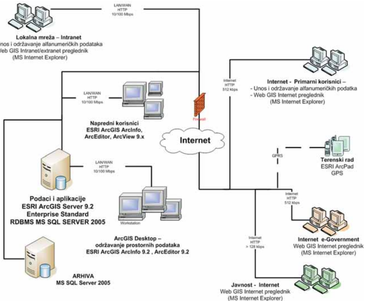
Fig. 1. Architecture of the GEOLIS digital base
