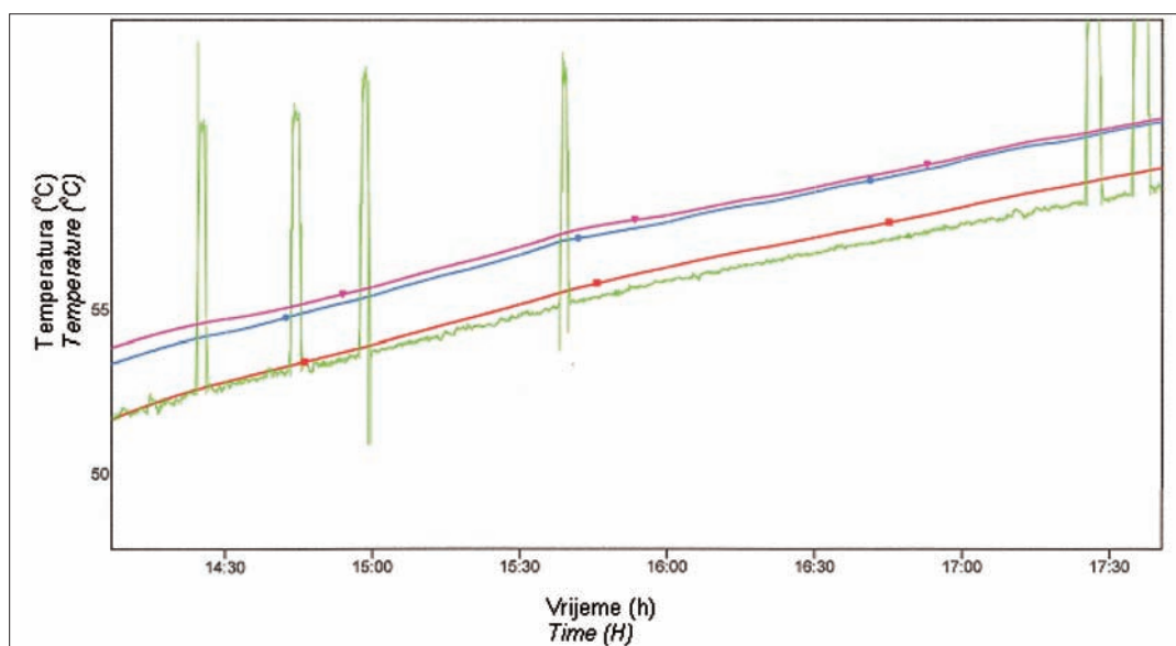
Slika 5. Nepravilan prikaz temperature mjerne sonde Figure 5 Improper display of temperature measuring probe
