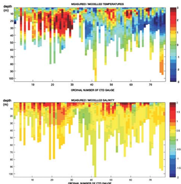
Figure 6 Difference of measured and model (ROMS) values (MEASURED - MODEL) for temperature (up) and salinity (down) on verticals of CTD measuring stations (July, 2008)
