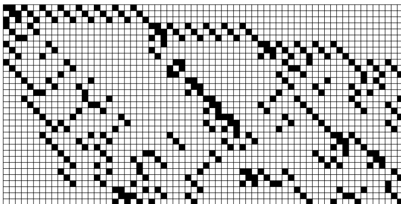
FIGURE 1. An incidence matrix of a \text{TSC}(4, 5) .
