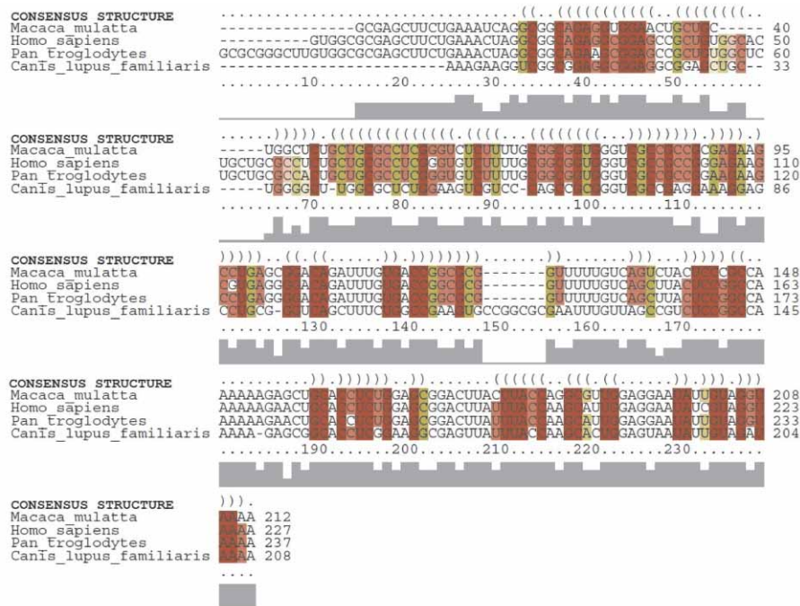
Figure 2. Structure annotated alignment. Consensus secondary structure of BRCA2 5' UTR based on alignment of sequences from four different species is presented in the first line in dot-bracket notation. Gray bars under the multiple sequence alignment present level of base conservation within that position in four 5' UTR sequences. The colors of the shadings indicate the number of different types of letter combinations that form a base pair. Red means that there is 1 and ochre that there are 2 different base-pair combinations. If a base pair cannot be formed in one or more sequences, the colors are shown faded in different levels.
