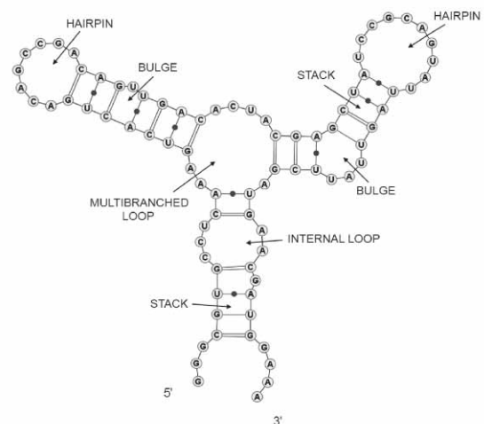
Figure 1. Elements of RNA secondary structure (base pairing). Each loop has at least one base pair. A stem consists of two or more consecutive stacks.
