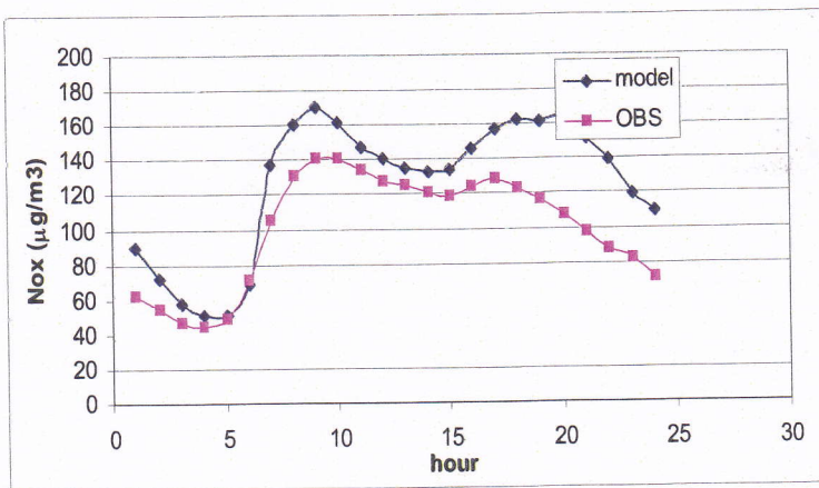
Figure 3. Average daily variation of NO 2 concentrations at street level in Franfurter (Berlin) compared with observations.
