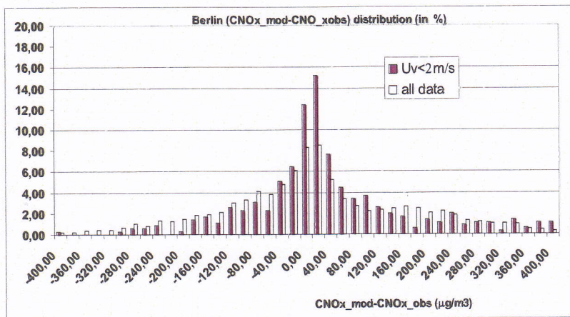
Figure 1. Error distribution, plain symbols for data at low wind speed ( <2ms^{-1} ), empty symbols for all data (Berlin Shildhornstrasse).
