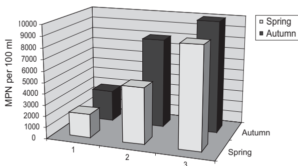
Figure 2 Mean total coliforms in the Sava River water samples by location and season.
