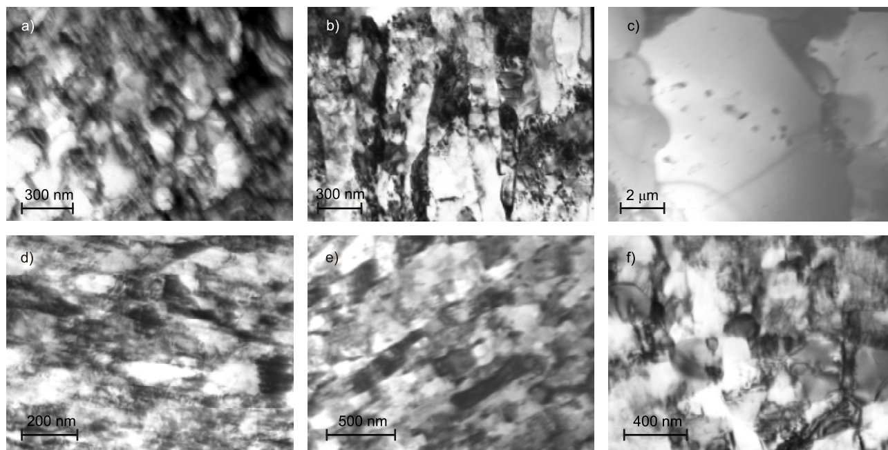
Figure 5. Structure of 0,1% C - 1,6 % Mn - 0,1 % V - 0,08 % Ti steel after cold ECA pressing and heating: a, d - ECAP; b - e - ECAP + 600 °C (10 min); c - f - ECAP + 700 °C (10 min); a - c - Initial ferritic-pearlitic state (before ECAP); d - f - Initial martensitic (bainitic) state (before ECAP)
