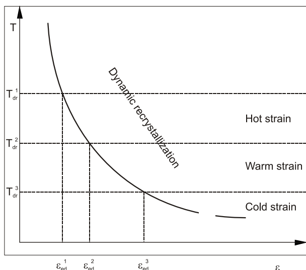
Figure 1. Dependence of critical strain for dynamic recrystallization on temperature
