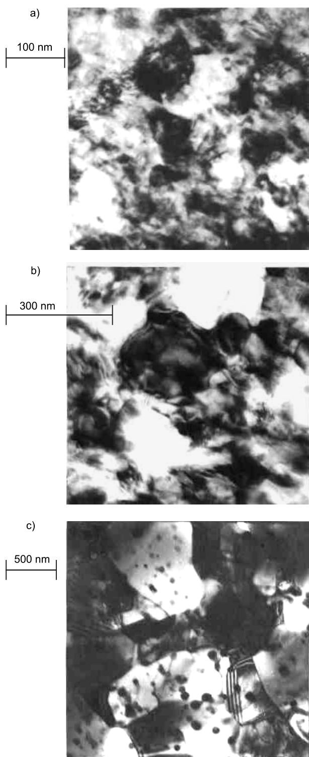
Figure 3. Structure of austenitic Cr-Ni-Ti steel after severe plastic deformation (SPD) by high pressure torsion: a - SPD, \epsilon = 6,3 (5 turns); b - SPD, \epsilon = 6,3 ; heating 500 °C (1 hour); c - SPD, \epsilon = 6,3 ; heating 700 °C (1 hour)
