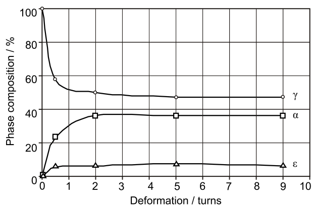
Figure 4. Changes of phase composition during SPD by high pressure torsion of austenitic 0,08 % C - 18,3 % Cr - 9,8 % Ni - 0,6 % Ti steel
