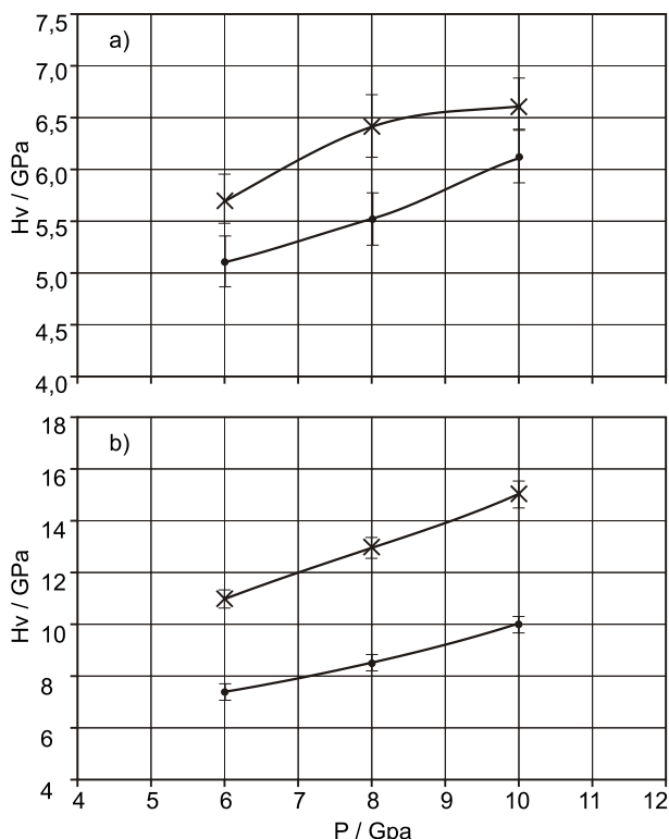
Figure 2. Microhardness dependence on pressure during SPD by high pressure torsion at room temperature with \epsilon \approx 6 . (Initial state: × - as-quenched, • - as-annealed): a - Low-carbon 0,1 % C - Mn - Si steel (S. Dobatkin et al, 2001); b - High-carbon 0,8 % C - 6 % W - 5 % Mo steel (S. Dobatkin, M. Zehetbauer et al, 2001)
