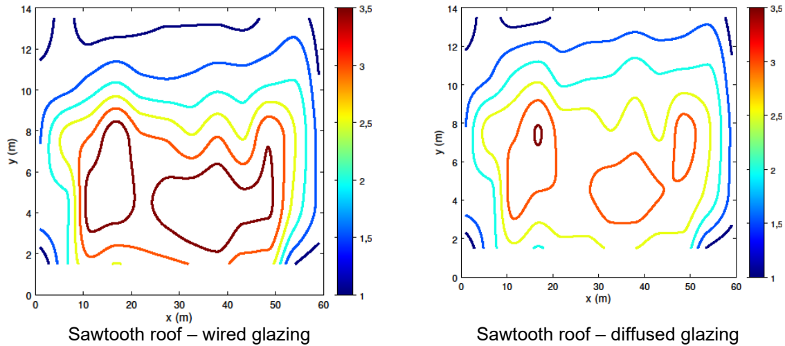
Figure 5. Plot of daylighting factor
