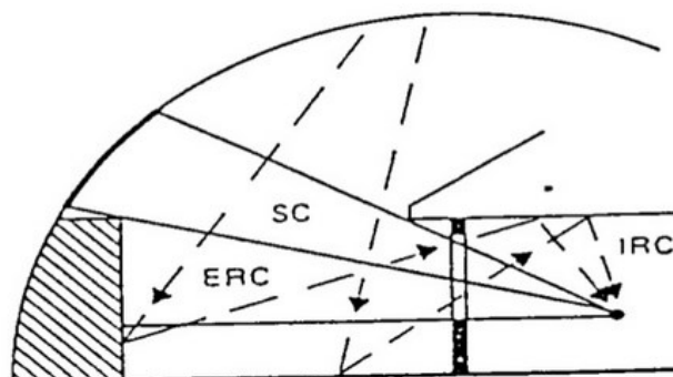
Figure 1. Daylight factor [4]
