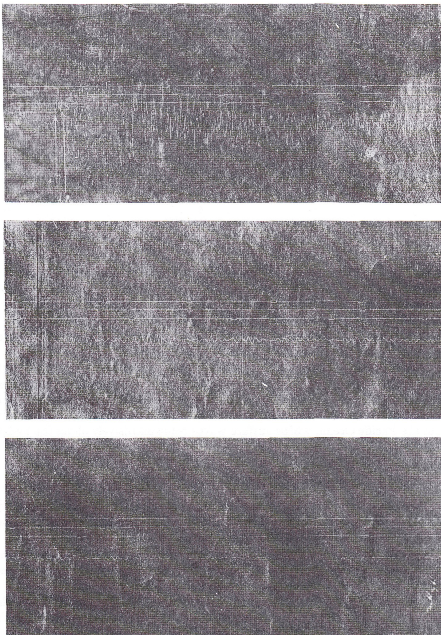
Figure 2. The earthquake of 8 October 1909 recorded at Zagreb. Magnification 20, NE component.
