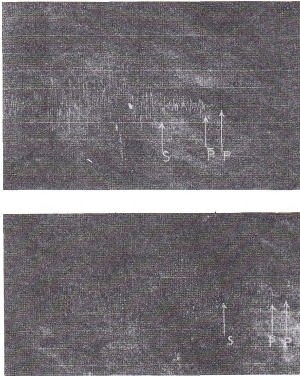
Figure 4. The earthquake of 25 August 1909. Sienna, a) Ne component, b) NW component.
