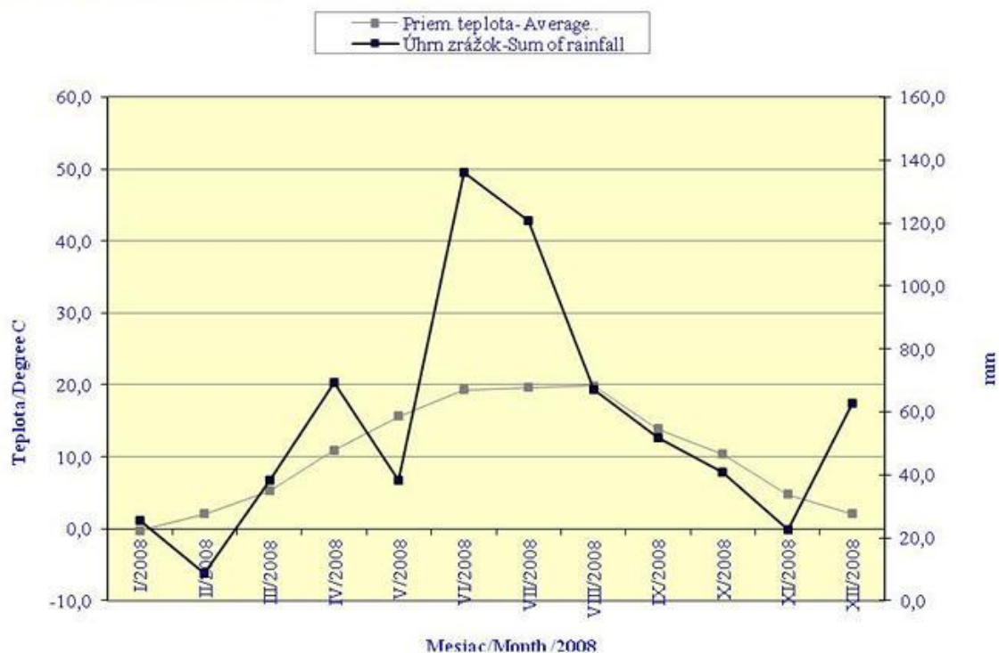
Graf 4: Walterov klimatogram 2008 Fig. 4: Walter's Climatogram 2008
