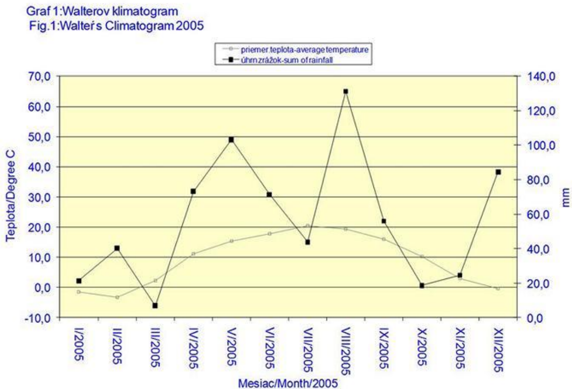
Figure 1. Walter's Climatogram 2005 Obrázok 1. Walterov klimatogram 2005
