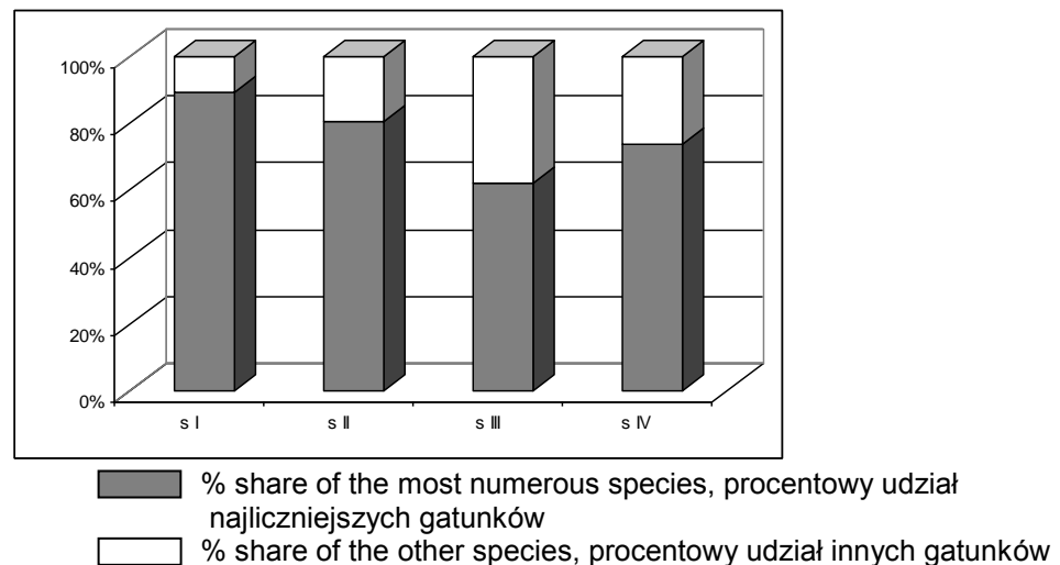
Figure 1. Percentage share of aphid species occurring in tested habitats: s I, s II, s III, s IV – see abbreviations in the text (1997-99)
