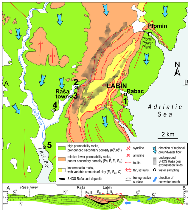
Figure 3: A simplified hydrogeological map with a cross section of the study area and its surroundings (Šikić et al., 1973). K_{2,1,2} – Turonian; K_{2,2,3} – Coniacian and Santonian/Campanian; Pc, E – Liburnian beds; E_1, E_{1,2} – Foraminiferal limestones; E_2 – Transitional beds; E_{2,3} – Flysch unit; Q – Quaternary.
