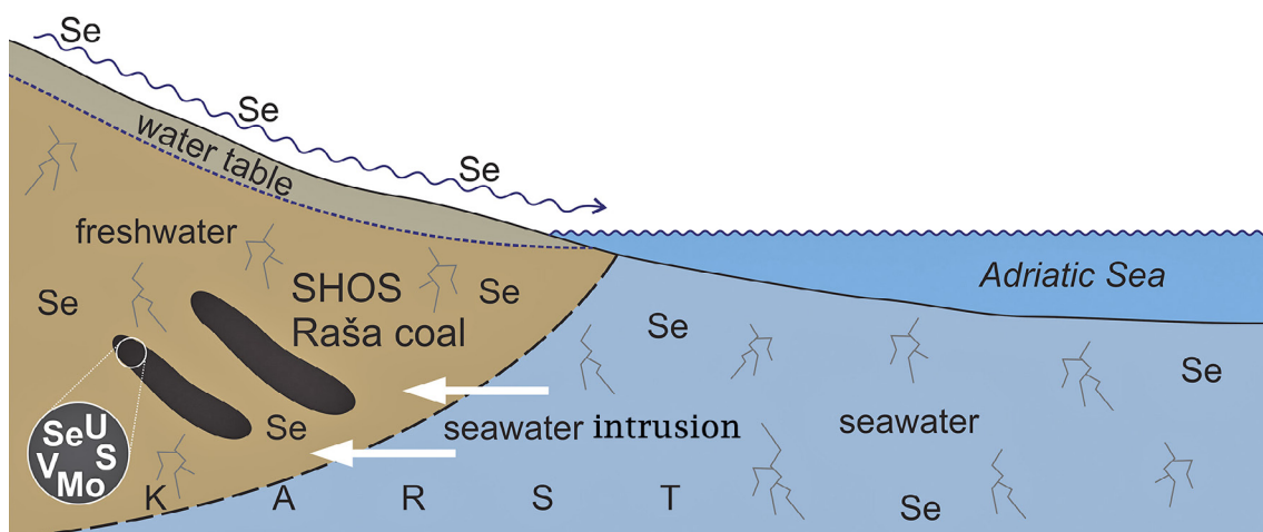
Figure 4: A scheme showing the mechanism of water-driven weathering of Raša coal in a karstic environment, and a concomitant enrichment of water with selenium derived from SHOS Raša coal.
