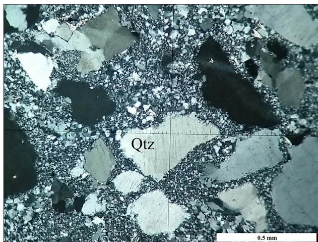
Figure 7: Microscopic photograph of the RK-5 quartz arenite (+ N). Poorly sorted quartz clasts in the finely grained quartz material, which could be formed chemically. Qtz = quartz.
