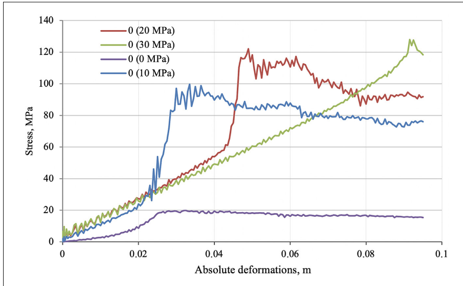
Figure 8: Tests of the jointed rock mass in 3D stress state at a 0° inclination angle of the main joint pattern
