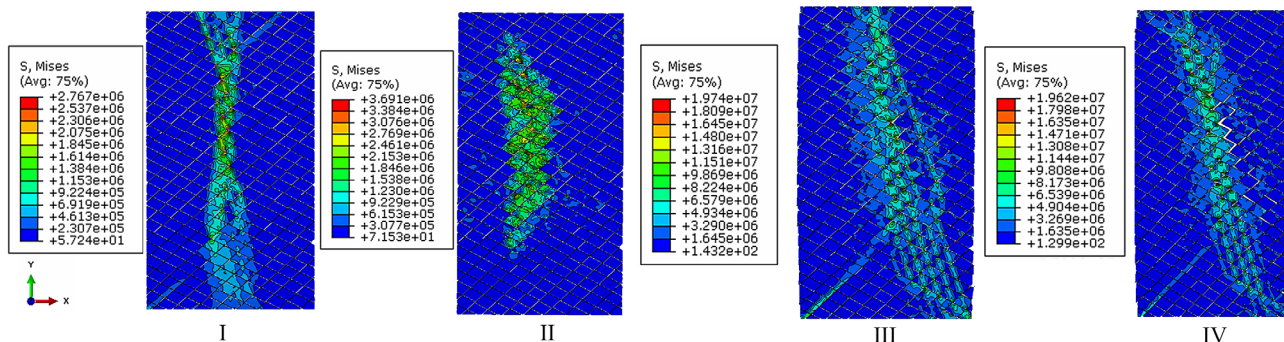
Figure 11: UCS virtual experiment stress-strain diagrams for the jointed rock mass with a 30° inclination angle of the main joint pattern where: I, II, III, IV are stages of deformations where 10%, 25%, 75%, 100% of the elastic deformations are realized accordingly
