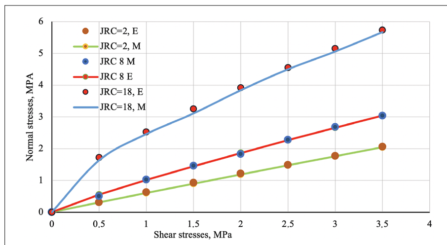
Figure 7: Certificate of rock strength in terms of interaction contact at various parameters of discontinuity roughness, where E: experimental results, M: simulation results of shear test
