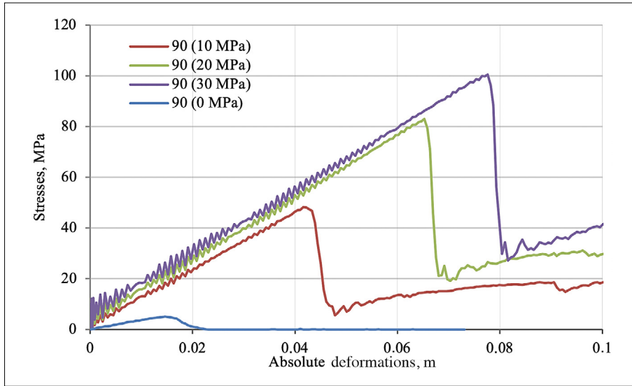
Figure 14: Tests of the jointed rock mass in 3D stress state at a 90° inclination angle of the main joint pattern
