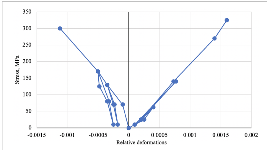
Figure 4: Uniaxial rock compression perpendicular to stratification
