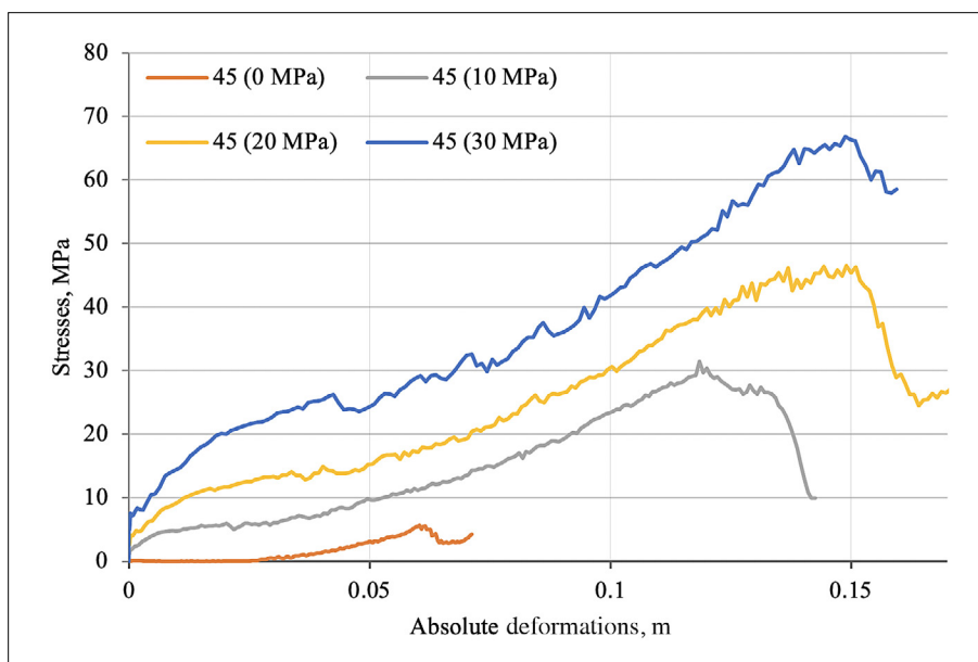
Figure 12: Tests of the jointed rock mass in 3D stress state at 45° inclination angle of the main joint pattern
