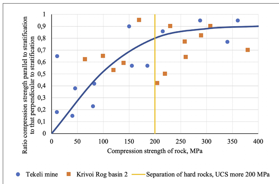
Figure 1: Variation of anisotropy coefficient of rock strength upon uniaxial compression
