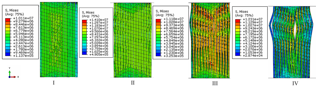
Figure 15: UCS virtual experiment stress-strain diagrams for the jointed rock mass with a 90° inclination angle of the main joint pattern where: I, II, III, IV are stages of deformations where 10%, 25%, 75%, 100% of the elastic deformations are realized accordingly
