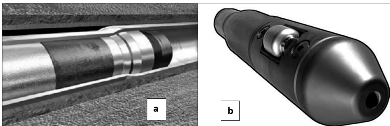
Figure 2: Fixed cone expander (a) and rotary compliant expansion tool (b) (Innes et al., 2004)
