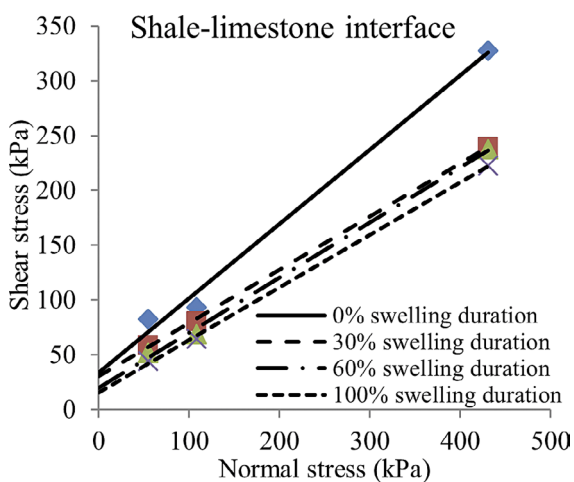
Figure 17: Shear strength envelope for shale-limestone interface at different swelling durations
