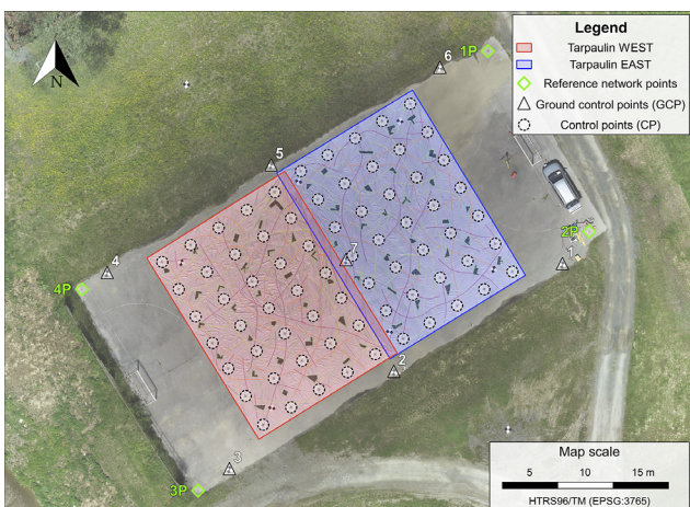
Figure 4: Distribution of the reference network points, CPs, and GCPs on tarpaulins
