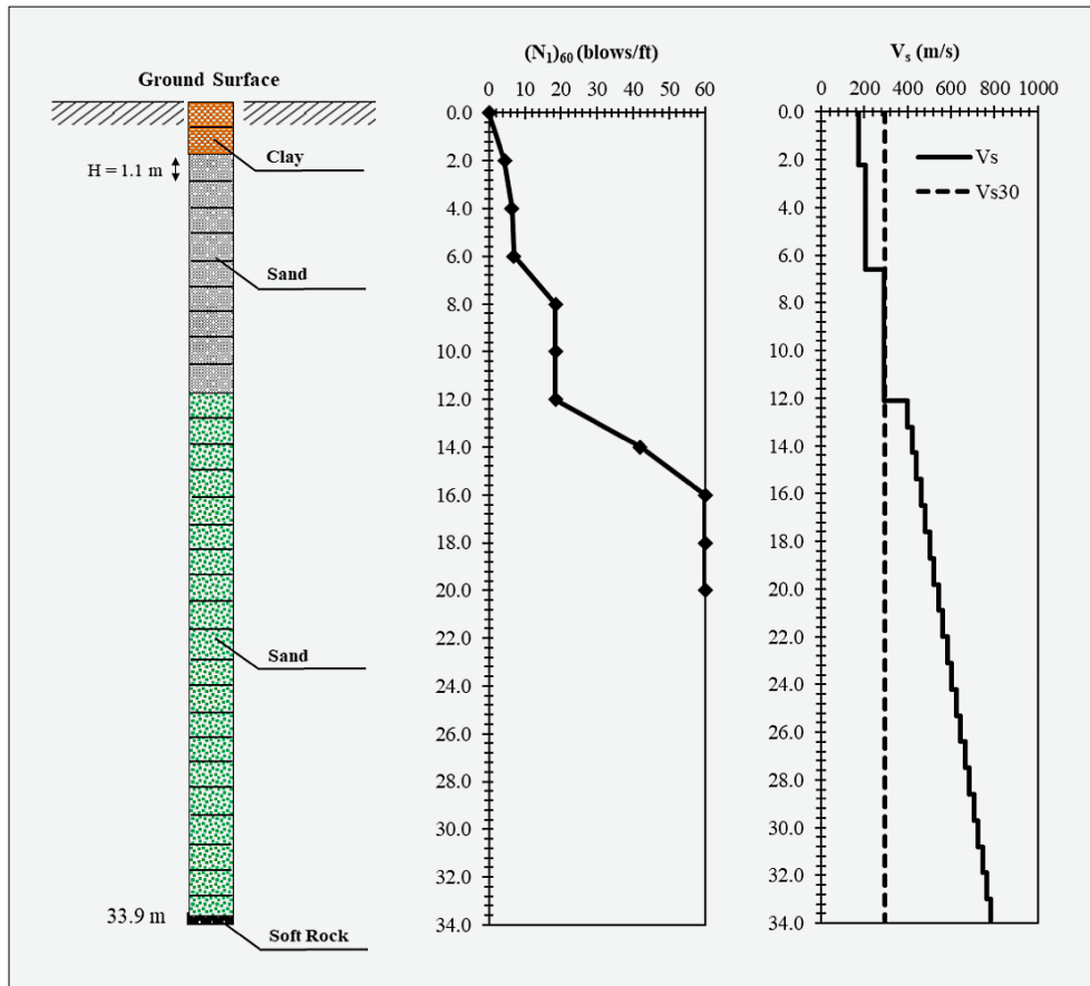
Figure 3: Condition of soil layers from site investigation
