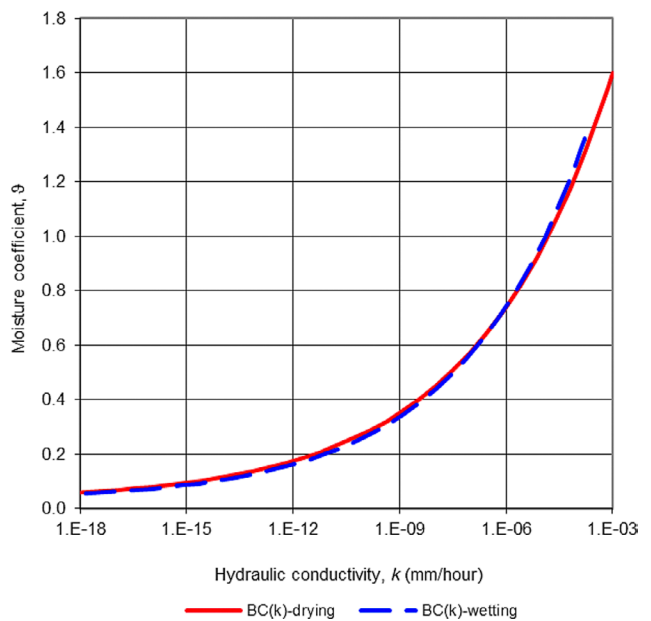
Figure 5: Hydraulic conductivity curves in drying and wetting in relation to moisture coefficient. Note: Data of BC(k)-drying curve are adopted from Kavur et al. (2011).
