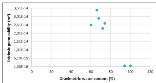
Figure 11. Gas permeability of porous media in relation to the gravimetric water content of samples (Pitanga et al., 2011)
