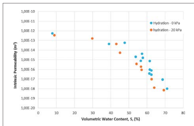
Figure 8. Gas permeability of porous media in relation to volumetric water content (Vangpaisal et al., 2002)
