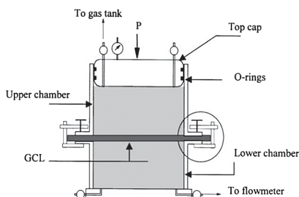
Figure 3. Gas permeability cell (Didier et al., 2000)
