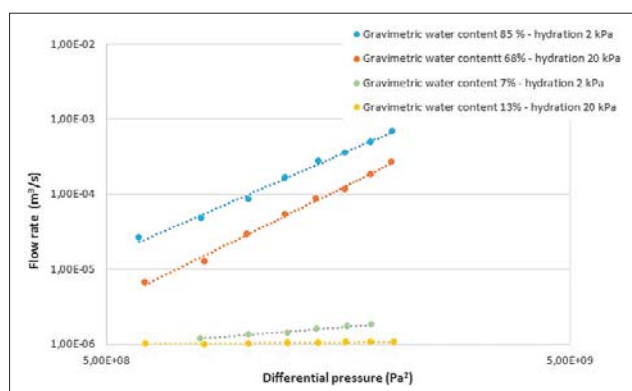
Figure 9. Gas flow rate in relation to differential pressure (Rouf et al., 2014)
