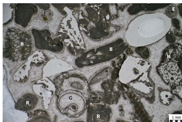
Figure 14: Algal-bryozoan grainstone with rhodoliths (R), Halimeda (H), bryozoans (B), gastropods (G) and echinoderms (E). Slide MB.8a, Stop T5.
