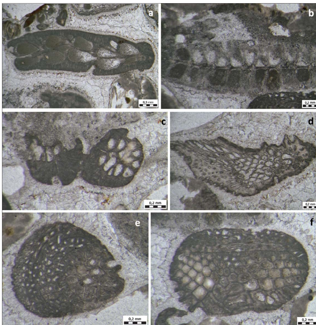
Figure 10: A variety of bryozoans present as bioclasts in bioclastic grainstone to rudstone at Marija Bistrica locality. Bifoliate ( a,b ) and branched ( c–f ) forms prevail in this microfacies. Thin sections MB.8a,b, Stop T5.
