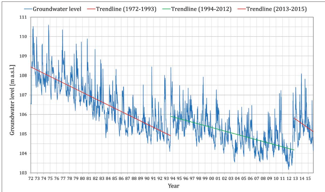
Figure 5: Negative trend of groundwater levels – observation well 107 located upstream from weir TE-TO, right bank of the Sava River
