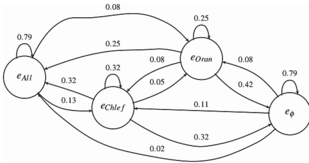
Figure 13: Obtained Markov chain
