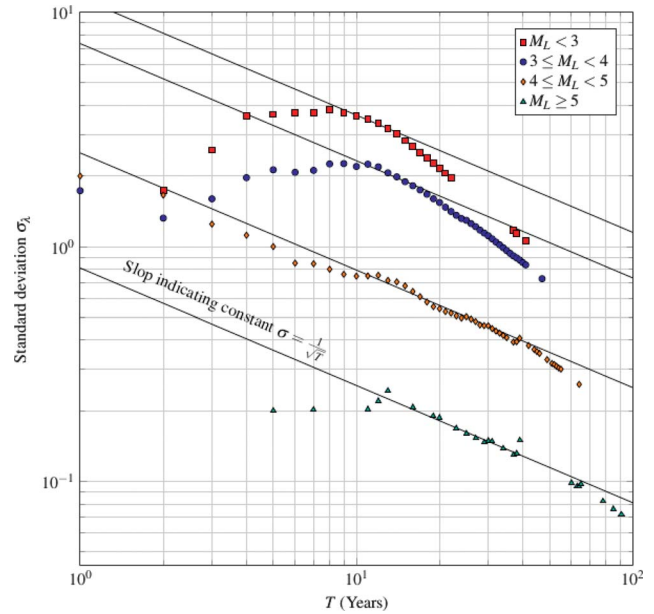
Figure 7: Completeness analysis based on the (Stepp, 1972) method
