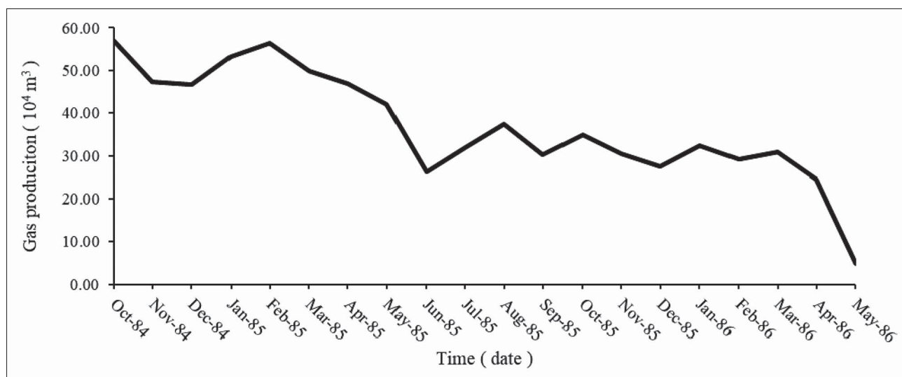
Figure 3: Monthly gas production for gas reservoir MALM.
