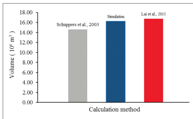
Figure 7: Cumulative injected \text{CO}_2 volumes obtained with two analytical methods (Schuppers et al., 2003; Lai et al., 2015) and with simulation done in ECLIPSE.
