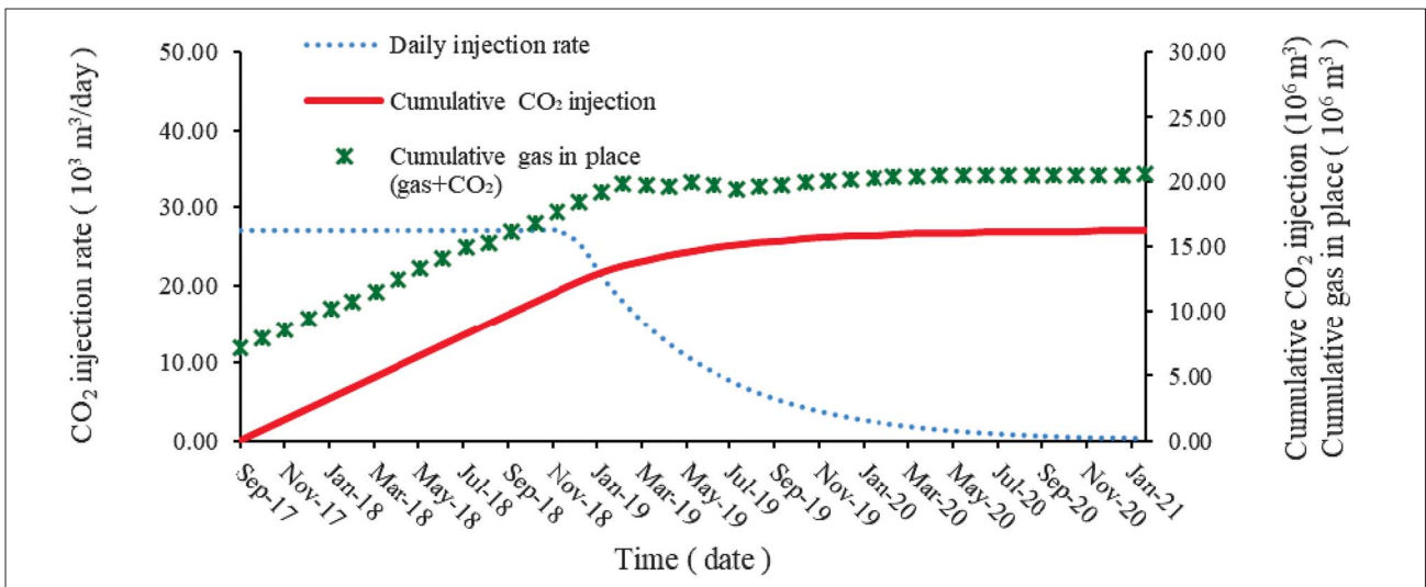
Figure 5: Cumulative CO 2 injection and gas in place.
