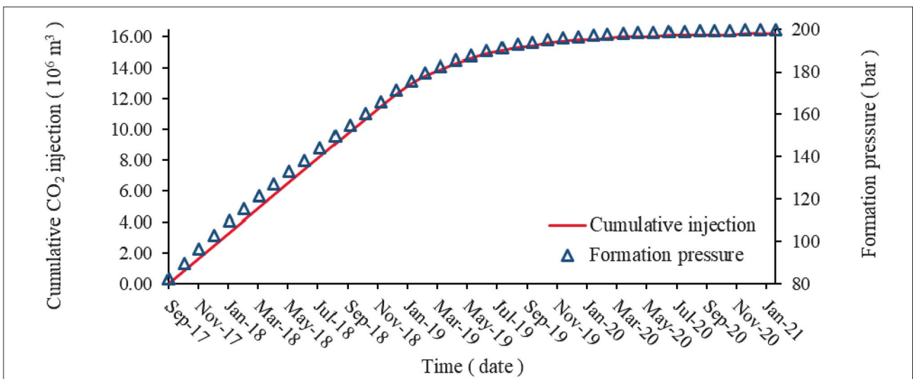
Figure 6: Formation pressure and cumulative CO 2 injection.
