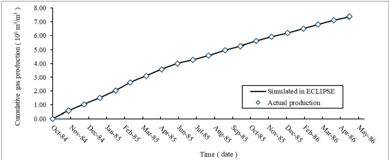
Figure 4: History matching of production.
