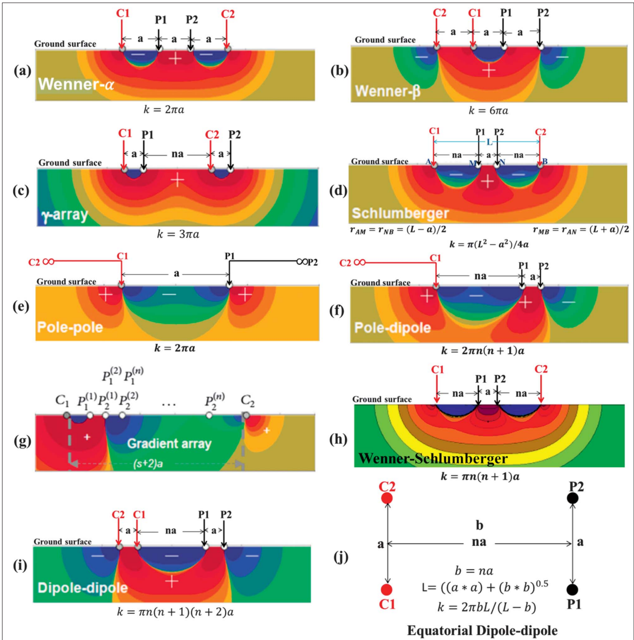
Figure 4: Array types with their respective configurations and geometric factors. C (1, 2) represents current electrode, P (1, 2) represents potential electrode, n is an integer value for dipole separation factor, a represents electrode spacing, k is the geometric factor, and \infty implies larger electrode separation of about 20 times the normal electrodes separation a . The background shows the sensitivity pattern of the configuration, in the gradient array case for the first potential electrode pair ( n -factor =1) (modified after Loke, 2002; Dahlin and Zhou, 2004).
