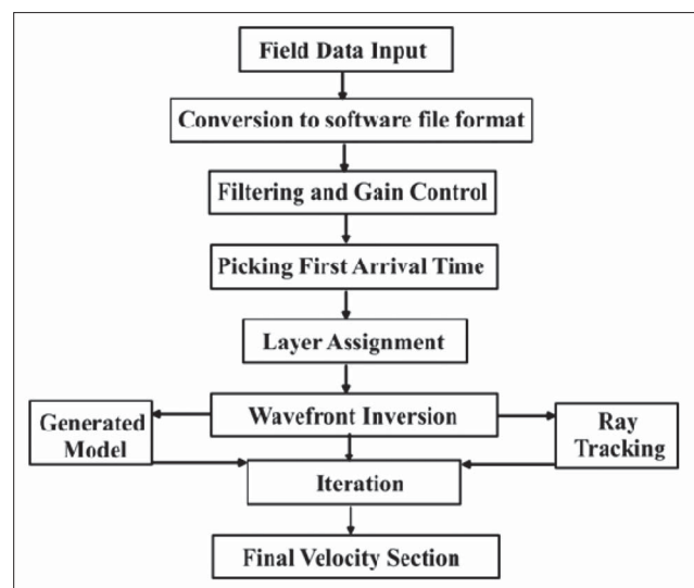
Figure 2: Seismic refraction tomography data processing flow chart.
