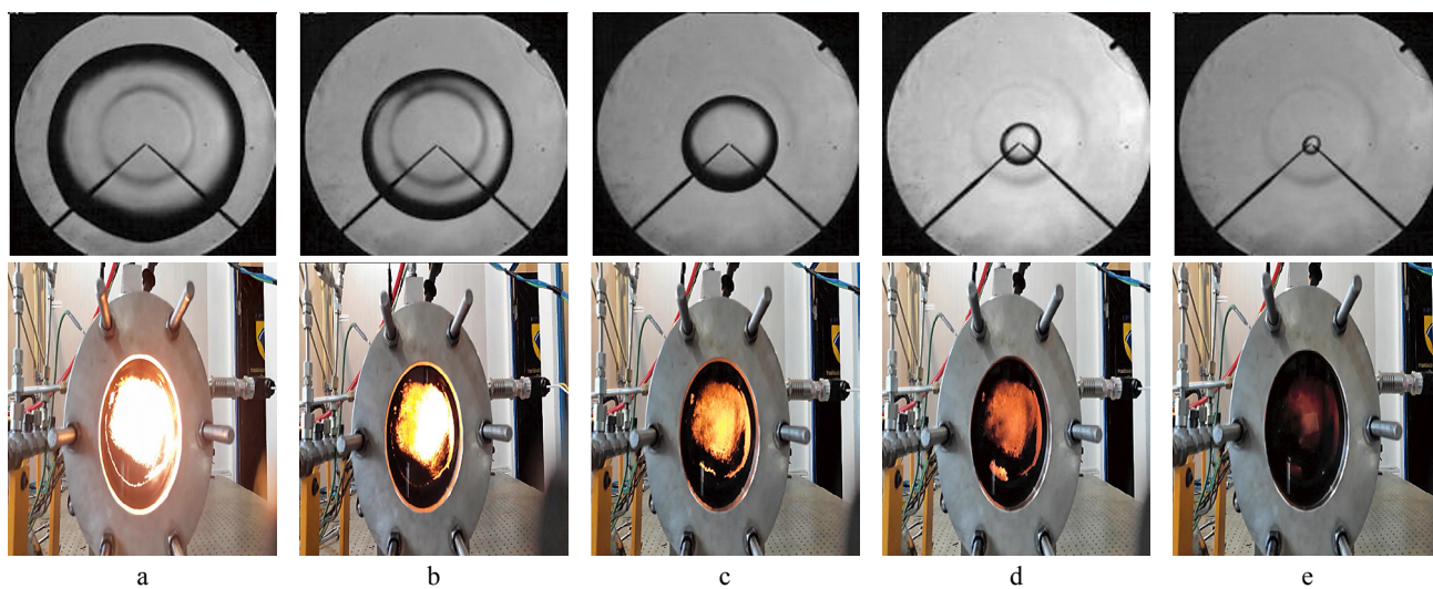
Figure 12: Spherical flame propagation process in each combustion cycle of methane and coal mixing
