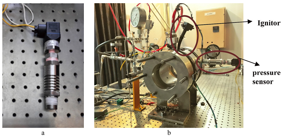
Figure 11: a) Pressure sensors used in coal dust explosion test; b) Pressure sensor mounted on the combustion chamber
