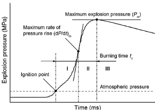
Figure 4: Profiles of various types of pressure in a coal dust explosion ( Li et al., 2018b )
