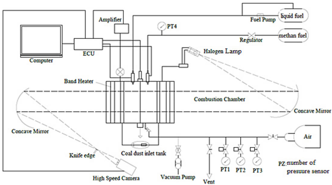
Figure 8: Schematic of the test layout
