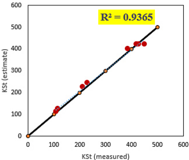
Figure 14: Comparison of measured and predicted values for relationship no.1 for testing data
