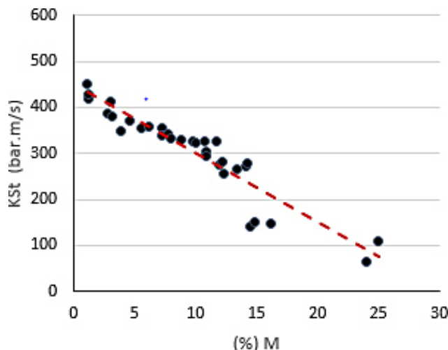
Figure 13: Variation of explosion index based on increased content of moisture
