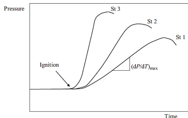
Figure 5: P Variation versus the time behavior with different St classes ( Wypych, 2001 ).
