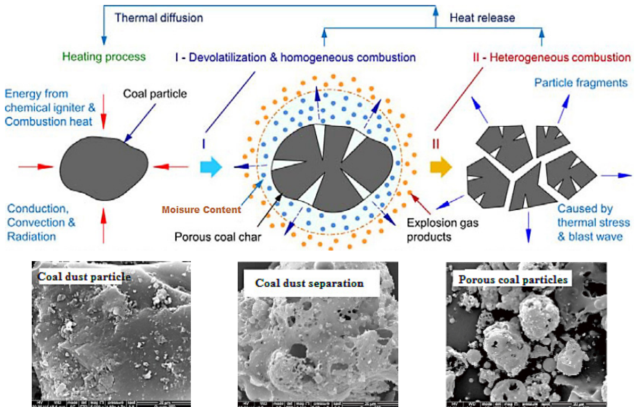
Figure 2: Changes in coal dust structure during the coal dust explosion process (Yuan et al., 2014).
