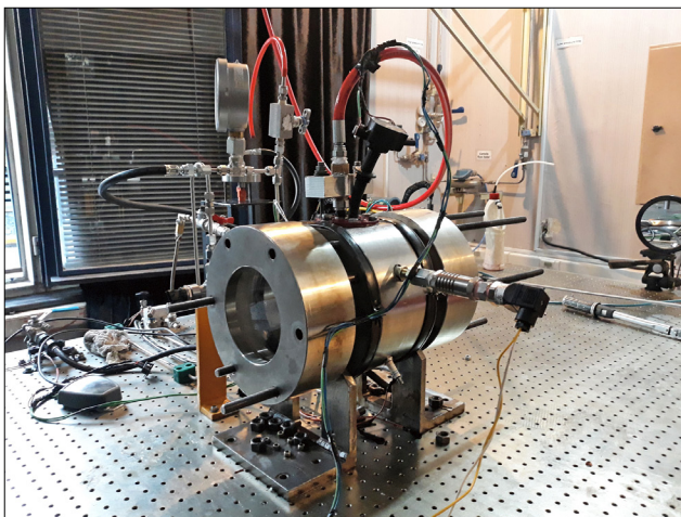
Figure 9: Real view of the equipment used in the coal dust explosion test
