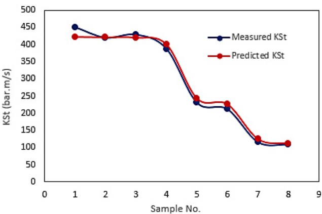
Figure 15: Comparison of the measured and predicted values of the K St test method for testing data
