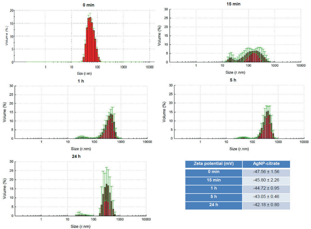
On-line Suppl. Fig. 1. Size distribution plots and zeta potentials of nanoparticles in 150 µM AgNPs exposure solution (liquid half strength MS medium) after 0 and 15 min as well as 1, 5 and 24 h.
